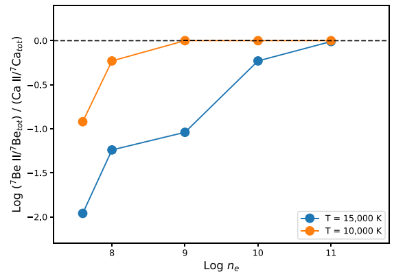
Figure 8. Relative mean ionization of {}^7\text{Be II} and \text{Ca II} , \log(\text{Be II}/\text{Be})/(\text{Ca II}/\text{Ca}) , for different values of gas densities and for two temperatures of the pseudo-photosphere.
