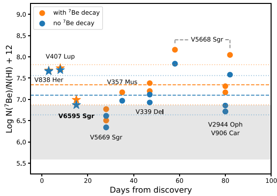
Figure 9. ^7\text{Be} abundances as a function of the day of observation with, in orange, and without correction for the ^7\text{Be} decay, in blue. The two ONe novae are shown with a star while the CO novae with a circle. The dashed lines mark the average value for both estimates. \log N(^7\text{Be})/N(\text{H}) + 12 = 7.34 \pm 0.47 when ^7\text{Be} decay is taken into account, and \log N(^7\text{Be})/N(\text{H}) + 12 = 7.10 \pm 0.46 , when it is not. The grey band shows the range of ^7\text{Be} yields for WD of different masses according to Starrfield et al. (2020). With this scale the meteoritic abundance is of A(^7\text{Li}) = 3.3 . The novae show a mean overabundance of four orders of magnitude (Lodders 2019).
