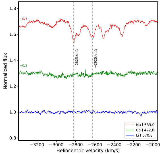
Figure 7. Spectra of April 16 in the regions of Na I 589.0 nm, Ca I 422.6 nm and {}^7\text{Li} I 670.8 nm. While blueshifted expanding absorptions are clearly detected for the Na I 589.0-nm line, there is no evidence of Ca I and {}^7\text{Li} I at the same expanding velocities. The absorptions of the D1 line are also visible redwards of the D2 line.
