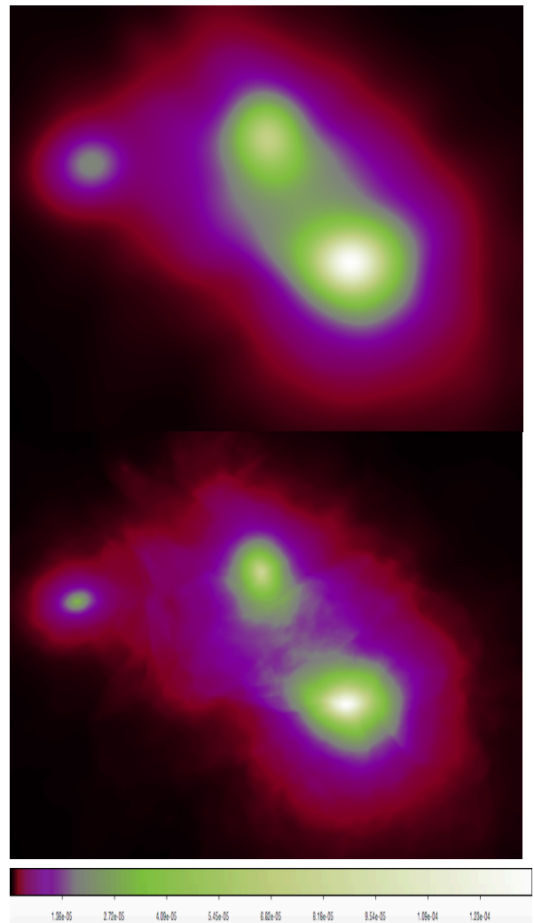
Figure 3. Simulated plasma signature within an A401–A399-like complex. The signal is in units of the Comptonization parameter \gamma reaching \sim 1.5 \times 10^{-4} in the clusters centers. Top: map of Comptonization parameter smoothed at the Planck resolution of 5'. Bottom: same map of the SZ signal at the resolution of \sim 10'' . The physical scale of each panel side is 7.5 Mpc.
