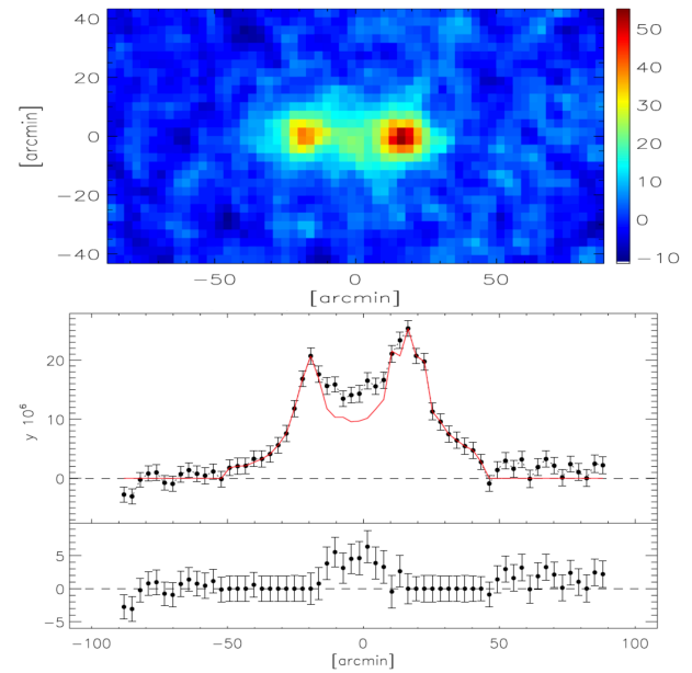
Figure 2. Top: map of Comptonization parameter ( y \times 10^6 ) as measured by Planck over the cluster pairs A401-A399. Bottom: y longitudinal profile (top part) and residual (bottom part) after subtracting the modeled contribution from the clusters (picture adapted from Planck collaboration, 2013).
