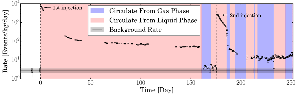
FIG. 1. Tritiated methane rate starting from the first injection. The left and right vertical black dashed lines represent the first and second tritium injection separately. The periods of circulating the xenon from the bulk liquid and from the gas phase are marked by the red and blue regions, respectively. The horizontal black solid line shows the background rate before tritium injection with the uncertainty in the rate, within 1\sigma , given by the black shaded region.
