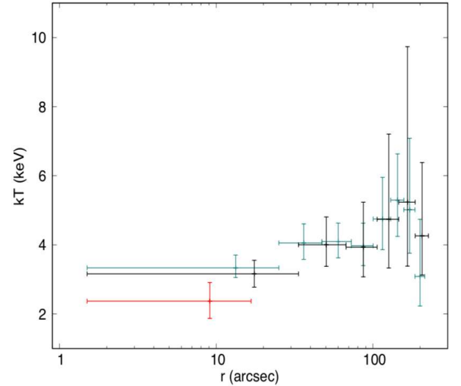
Figure 6. Projected (cyan) and deprojected (black) temperature profile of A2495. Bars in the x-axis represent the limits of the extraction rings, while the y-axis ones are the errors for the temperature values. The red point is derived from the spectral analysis described in Sec. 4.3.
