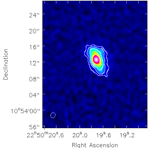
Figure 1. 5 GHz map ( ROBUST 0 ) of A2495. The resolution is 1.30'' \times 1.15'' , with a RMS noise of 4 \mu\text{Jy beam}^{-1} . Contours are at -3, 3, 6, 12, 24, 48 \cdot \text{RMS} . The source flux is 2.37 \pm 0.19 \text{ mJy} . The bottom-left circle represents the beam.
