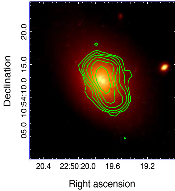
Figure 2. 1.4 GHz contours (ROBUST 0) of the radio source overlaid on an HST image (F606W filter) of A2495. The resolution of the radio map is 1.29'' \times 1.12'' , with a RMS noise of 10 \mu\text{Jy beam}^{-1} . Countours are at -3, 3, 6, 12, 24, 48 \cdot \text{RMS} . The source flux is 15.7 \pm 1.3 \text{ mJy} .
