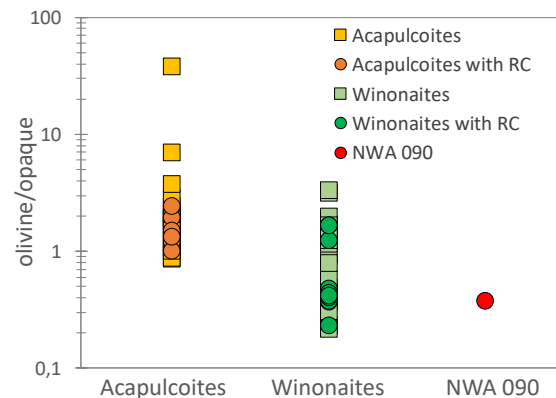
Fig. 2 – Ratio of modal olivine and opaque phases in acapulcoites and winonaite, with or without relict chondrules (RC). NWA 090 lies clearly in the winonaite range.
