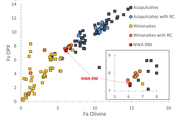
Fig. 3 – Ferrosilite content of low-Ca pyroxene vs fayalite content in olivine of acapulcoites and winonaite, with or without relict chondrules (RC).
