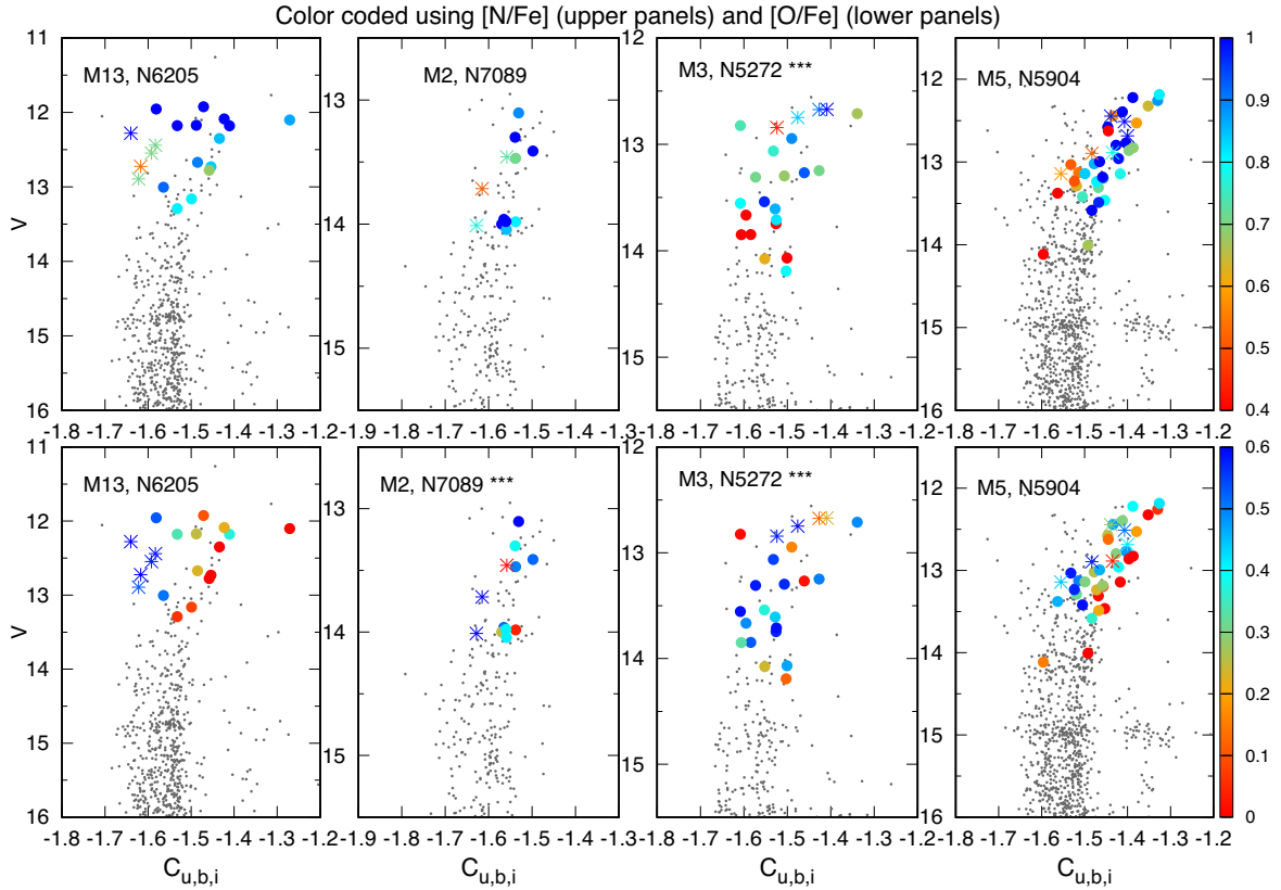
Figure 3. V - C_{U,B,I} diagram colour coded by [N/Fe] (upper panels) and [O/Fe] (lower panels) similarly to what can be seen in Fig. 2. Clusters with [M/H] < -1.8 are not plotted, because the uncertainties of [N/Fe] and [O/Fe] are high (Mészáros et al. 2015).
