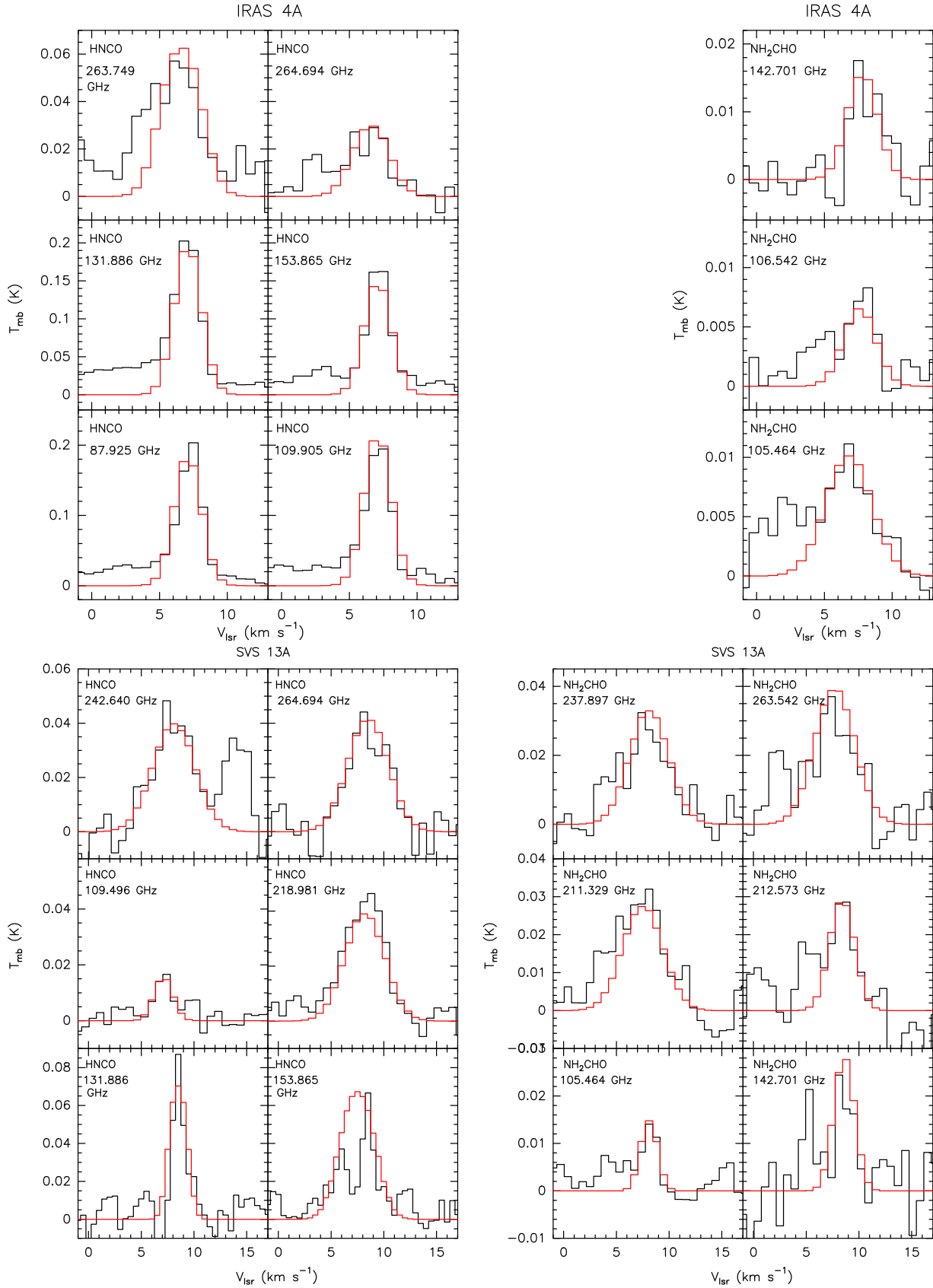
Figure C2. Sample of HNC ( left ) and NH 2 CHO ( right ) observed spectral lines (black) in IRAS 4A and SVS13A (compact solution), and the spectra predicted by best fit LTE model (red).
