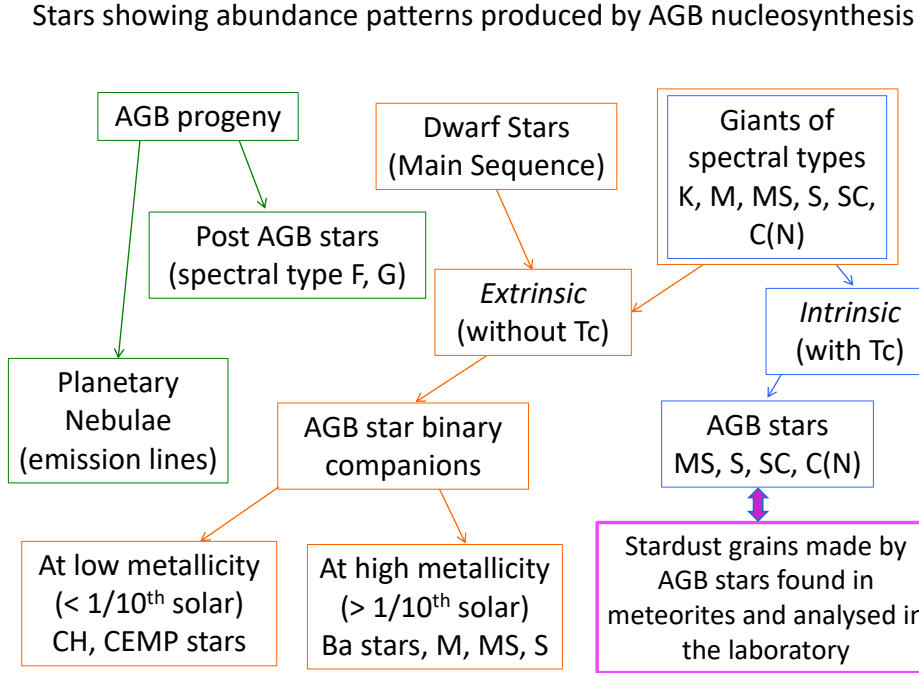
Figure 2. Schematic illustration of the different types of stars that show s -process enhancements: direct observation of AGB stars (blue arrows), or their progeny (green arrows), and binary enrichment (orange arrows). See Ref. [69] for a map between the spectral type and evolutionary phase of an AGB star. Stardust grains represent another direct link, as they formed around AGB stars.
