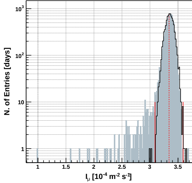
FIG. 4. Distribution of the daily muon flux (grey histogram). The dashed red line represents the mean value. The black histogram represents the distribution expected from the temperature variations taking into account the expected correlation coefficient as well as the statistical and systematic uncertainties on the muon flux. The two continuous lines define the flux limits within which data are used.
