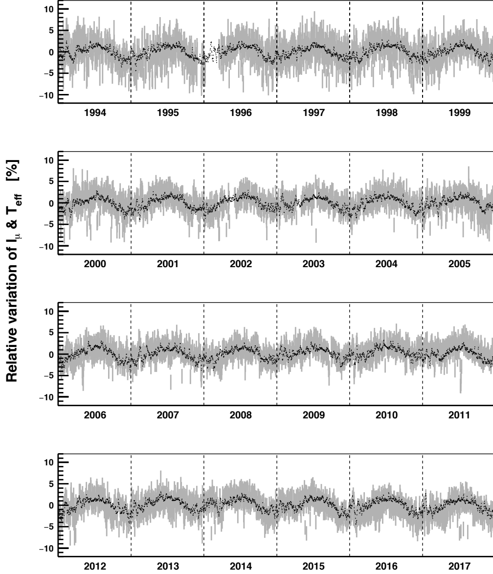
FIG. 5. Grey histogram: percent variations of the daily muon flux, \Delta I_\mu/I_\mu^0 as a function of time. The error bars represent the statistical uncertainty. Black points: percent variations of the daily effective temperature, \Delta T_{\text{eff}}/T_{\text{eff}}^0 , as a function of time.
