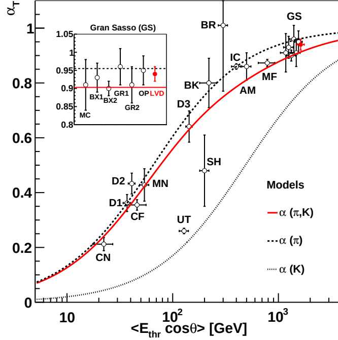
FIG. 7. Comparison of the experimental \alpha_T values with the models [34] accounting for pions and kaons decays (solid red line), pions decays only (dashed black line) and kaons decays only (dotted black line). The value determined in this work is reported as a filled red point, the error bar corresponding to the sum of the statistical and systematic uncertainties. The open points represent the values determined by other experiments: Amanda (AM) [19], Baksan (BK) [18], Barrett (BR) [12], the three experimental halls of Daya Bay (D1, D2 and D3) [25], Icecube (IC) [20], MINOS Near (MN) [21] and Far (MF) [30] detectors, Double Chooz Near (CN) and Far (CF) detectors [24], Sherman (SH) [16], and Utah (UT) [17]. The six Gran Sasso (GS) based measurements are highlighted in the inset and include MACRO (MC) [5], Borexino (BX1 and BX2) [33],[26], GERDA (GR1 and GR2) [22], Opera (OP) [23] and LVD (this work). They are artificially displaced on the horizontal axis for a better visualization.
