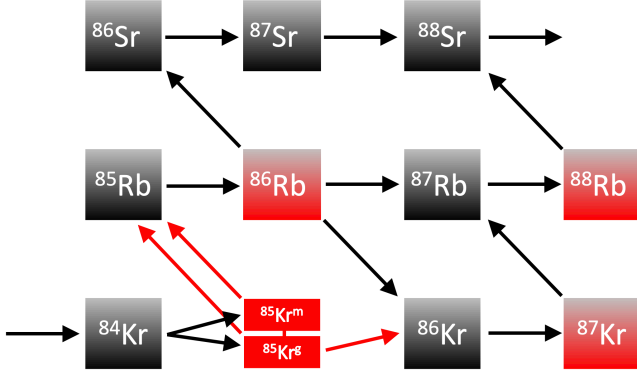
Figure 4. The s-process nucleosynthesis path in the region around N = 50 ; the ^{85}\text{Kr} branching is highlighted by the red arrows. Stable isotopes are shown in black boxes while unstable ones have a red background.
