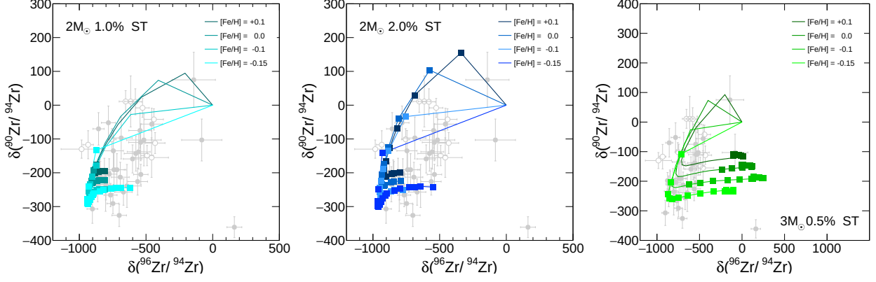
Figure 21. The comparison of measured SiC data involving ^{90}\text{Zr} with model sequences for the winds of 2 M_{\odot} stars at 1% and 2% dilution of He-shell matter in the winds (left and center panels) and for those of 3 M_{\odot} stars with a low percentage (0.5%) of He-shell matter added (right panel).
