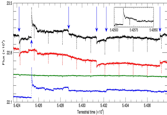
Fig. 7. Light curves of an eclipsing binary that displays a series of discontinuities indicated by blue arrows. The colour code corresponds to the three colour light curves, with the resulting white light curve plotted in black. We note that the colour light curves have been shifted by a constant in order to avoid too large a scale on the y axis. The top inset is a magnification of a portion of the light curve where the discontinuity in flux is not a simple step but a sudden increase of the flux, followed by an exponential decrease as could be generated by the impact of a proton on the CCD.
