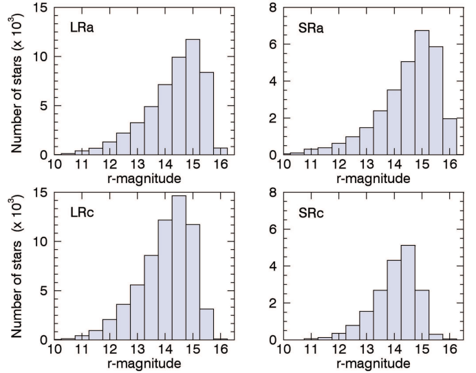
Fig. 2. Distribution of r -magnitude for the stars observed in the long runs and short runs in the anticentre (top) and centre (bottom).
