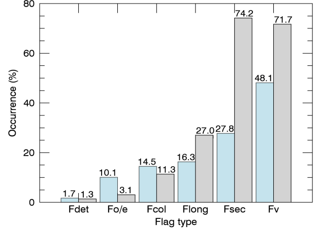
Fig. 15. Occurrence in percentage of each flag (see Sect. 3.5) for the candidates (blue) and the EBs (grey).
