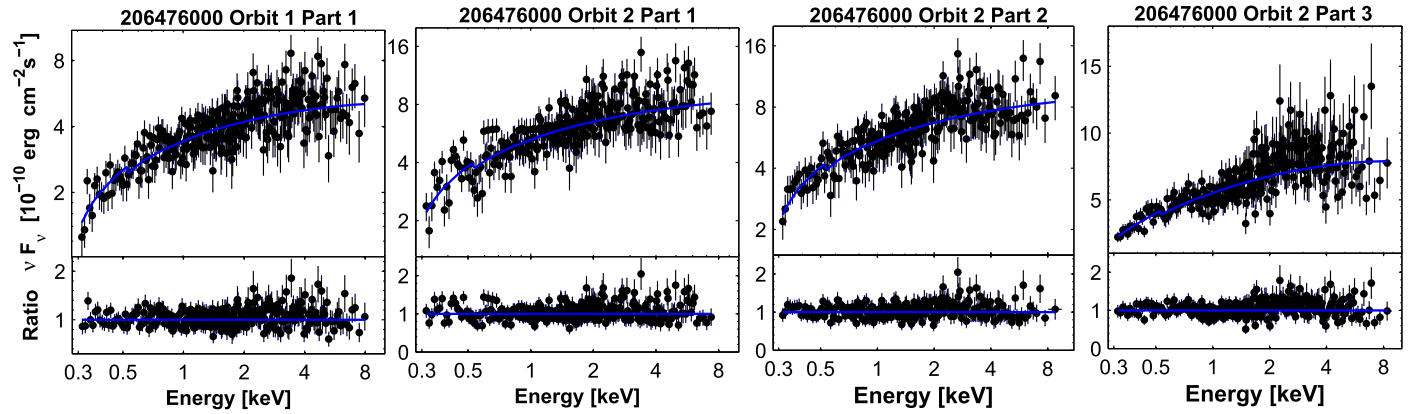
Figure 3. Log-parabolic spectra yielding E_p > 10 keV, along with the distribution of the residuals. In each spectrum, a solid line represents the log-normal model defined by Equation (2).
