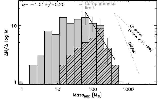
Fig. 2. Mass distribution of MDCs within d \leq 4.5 kpc. The Poisson error of each bin is shown as a grey line above the 10\sigma_{\text{rms}} completeness limit of 50 M_\odot , the power-law fit is shown in a solid black line. Hashed area shows the distribution of the brightest cores ( M_{\text{MDC}}^{\text{max}} ) per clump. Dashed lines show the slope of the CMF/IMF (André et al. 2014) and CO clumps (Kramer et al. 1998).
