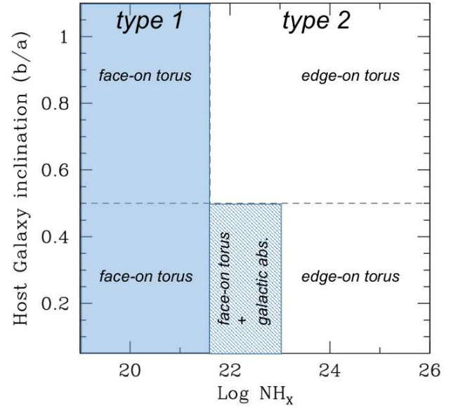
Fig. 4. Scheme of the expected type of absorption in the b/a - N_H plane for broad line (left blue side) and narrow line AGN (right side) in relation to the torus and host galaxy misalignment. The dashed blue region represents values where a type 1 AGN could be likely classified as type 2 due to absorption located in the host galaxy.
