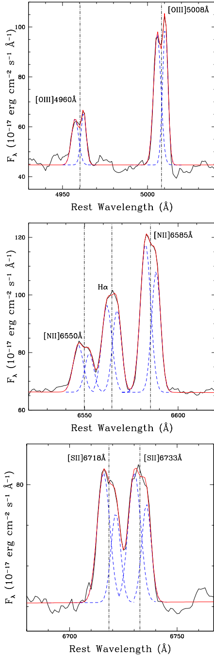
Figure 2. MCG+11-11-032 rest-frame spectrum around the [OIII] (top panel), H\alpha + [NII] (middle panel) and [SII] (bottom panel) regions. Wavelengths are in vacuum. Red solid lines represent the total fit, while blue dashed lines are the gaussian components. Black dot-dashed vertical lines mark the position of the line at the systemic velocity of the host galaxy.
