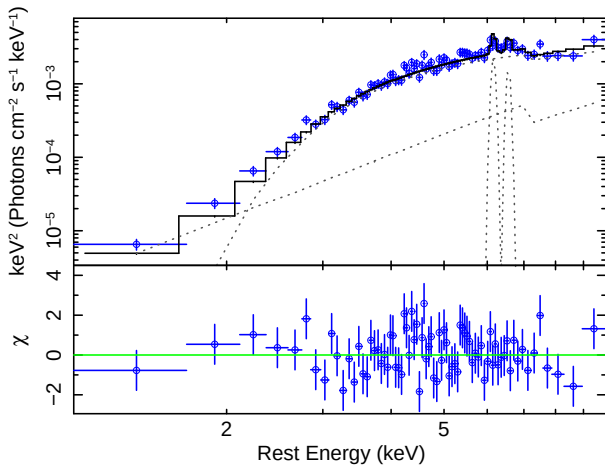
Figure 9. Upper panel: the model, which includes an intrinsically absorbed power-law plus a continuum reflection component and two emission narrow lines ( tbabs*(ztbabs*zpowerlw+pearrav+zgauss+zgauss) ), model 4 in Table 3, is plotted over the spectrum of MCG+11-11-032. Note that this plot was obtained by creating fluxed spectrum against a simple \Gamma = 2 power-law and then overlaying the best fit model. Lower panel: relevant residuals, plotted in terms of sigmas.
