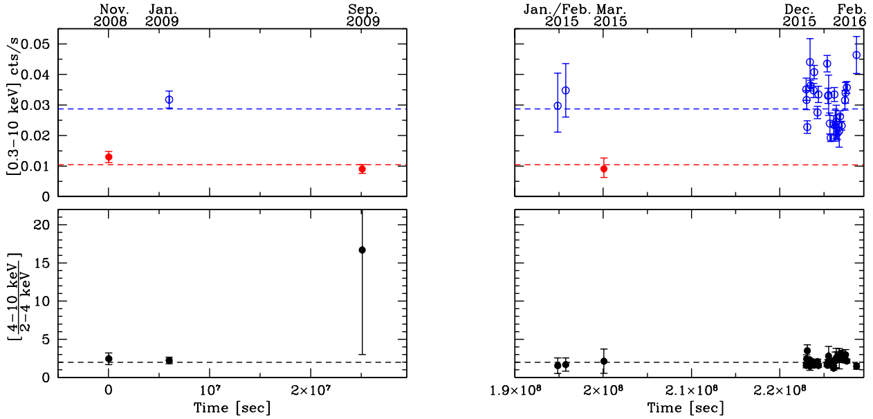
Figure 3. 0.3-10 keV XRT count rate (upper panels) and hardness ratio (lower panels) light curves of MCG+11-11-032 obtained by binning the data per observation. Data points are corrected for technical issues (i.e. bad pixels/columns, field of view effects and source counts landing outside the extraction region) following the recipes discussed by Evans et al. (2007, 2009) . Error bars mark 1\sigma uncertainties, while dashed lines represent the weighted averages of the high and low count rate states (upper panels, blue and red lines, respectively) and of the hardness ratios (lower panels, black line). In the upper panels, blue and red points flag higher and lower count rate states, respectively.
