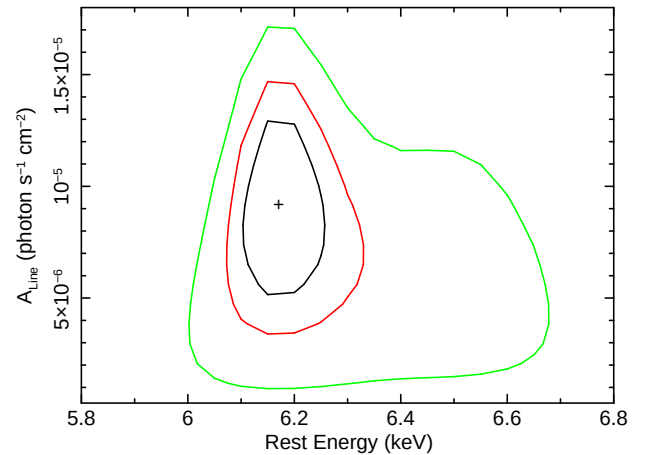
Figure 8. Confidence contours plot of the joint errors of the rest-frame emission line energy versus the intrinsic normalization of the Gaussian component ( A_{line} ). 68 per cent (black line), 90 per cent (red line) and 99 per cent (green line) confidence contours are shown.
