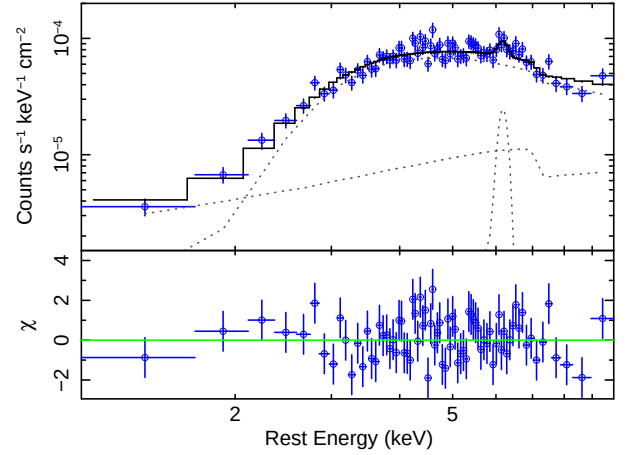
Figure 7. Upper panel: The model composed of an intrinsically absorbed power-law plus a continuum reflection component and one narrow emission line ( tbabs*(ztbabs*zpowerlw+peirav+zgauss) , model 3 in Table 3) is plotted over the XRT spectrum of MCG+11-11-032. Lower panel: Relevant residuals plotted in terms of sigmas.
