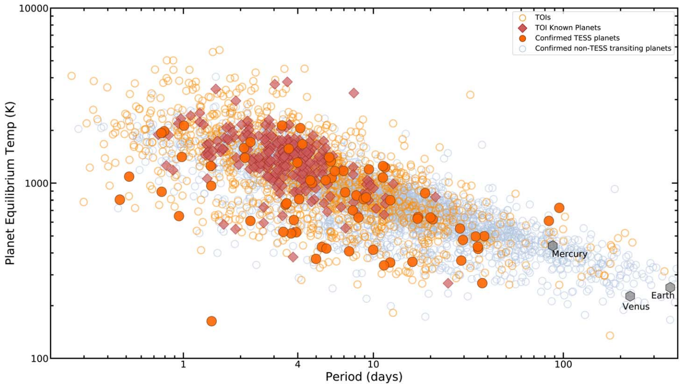
Figure 11. Orbital period vs. planet equilibrium temperature. The planet orbital period in days is on the horizontal axis, and the planet T_{\text{eq}} is on the vertical axis. The open orange circles are planet candidate TOIs that have not been confirmed. The filled orange circles are planets that are either confirmed with a mass measurement or validated by other means. The red diamonds are TOIs that were known planets prior to the TESS mission. The blue open circles are known planets from outside the TESS mission (NASA Exoplanet Archive, accessed 2020 October 8). Mercury, Venus, and Earth are visible in the bottom right. The TOI catalog has greatly increased the number of temperate short-period planet candidates available for follow-up.
