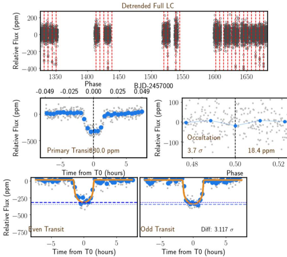
Figure 3. The QLP DV summary report plots for \pi Men c (Huang et al. 2018b). Top row: detrended full light curve with all available sectors stitched together. Transits are marked by red vertical lines. Middle row left: phase-folded light curve. The gray points are all data points, and the blue points are binned relative to the transit window size to guide the eye. Middle row right: phase-folded light curve at phase 0.5 for a secondary eclipse test. Bottom row: even and odd transits. The model fit is shown in orange. The depths of even transits are marked by darker dashed lines and odd transits by lighter dashed lines. A significant difference in the depths ( >5\sigma ) would suggest that the TCE is an EB at twice the period. Right-hand column: planet and stellar parameters.
