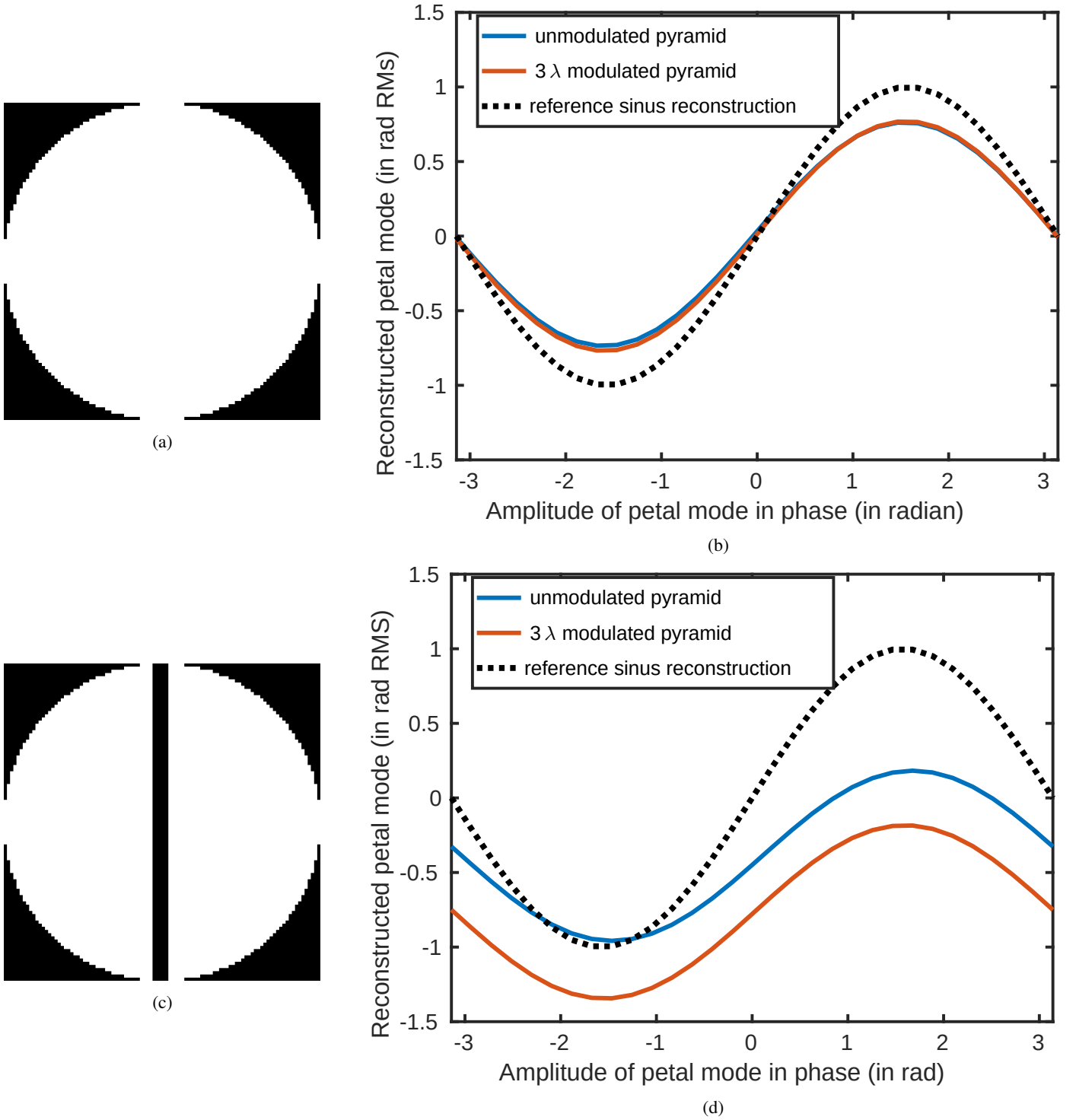
Fig. 4: Linearity curve in presence of residuals for unobstructed pupil and toymodel pupil. Fig. a) : Unobstructed pupil. Fig. b) : Linearity curve of petal mode around residual phase screen for unobstructed pupil. Fig. c): Obstructed pupil. Fig.d) : Linearity curve of petal mode around residual phase screen for toymodel pupil
