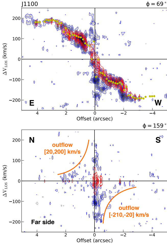
Fig. 8. Same as in Fig. 6 but for J1100. The CO kinematic major axis is PA = 69^\circ , the minor axis PA \sim 159^\circ = -21^\circ and the inclination i = 38^\circ . We used a slit width of \sim 0.2'' .
