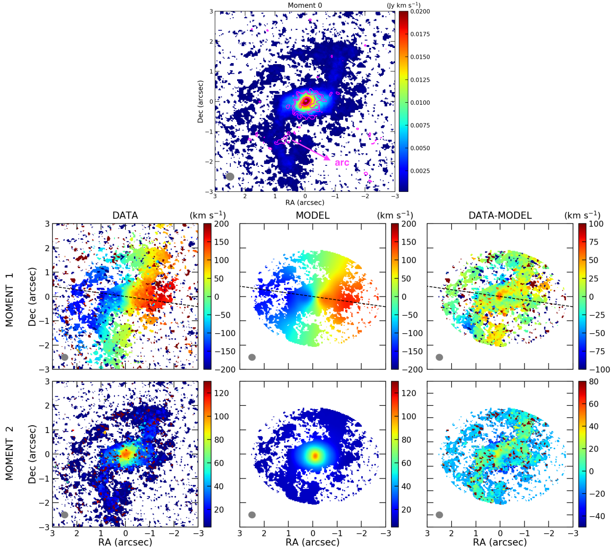
Fig. 13. Same as in Fig. 5 but for J1509. Continuum contours starting at 3\sigma are shown in pink in the moment 0 map ( \sigma = 0.013 mJy beam ^{-1} ), and beam size is 0.26'' \times 0.24'' .
