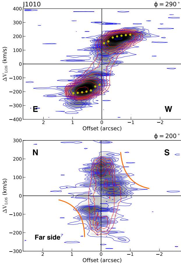
Fig. 6. PV diagrams along the CO kinematic major axis ( PA = 290^\circ = -70^\circ ) and minor axis ( PA = 200^\circ = 20^\circ ) of J1010 extracted with 3D BAROLO. We used a slit width of \sim 0.8'' . Blue contours correspond to the observed CO(2–1) emission above 2\sigma and red contours to the 3D BAROLO rotating disk model (inclination of i = 36^\circ ) shown in Fig. 5. Yellow dots are the average model velocities at different radii. Blue contours outside the boundaries of the model correspond to noncircular motions. Orange lines indicate the positive/negative pattern that, in the case of this QSO2, might be produced by either a coplanar inflow or a spatially extended vertical outflow.
