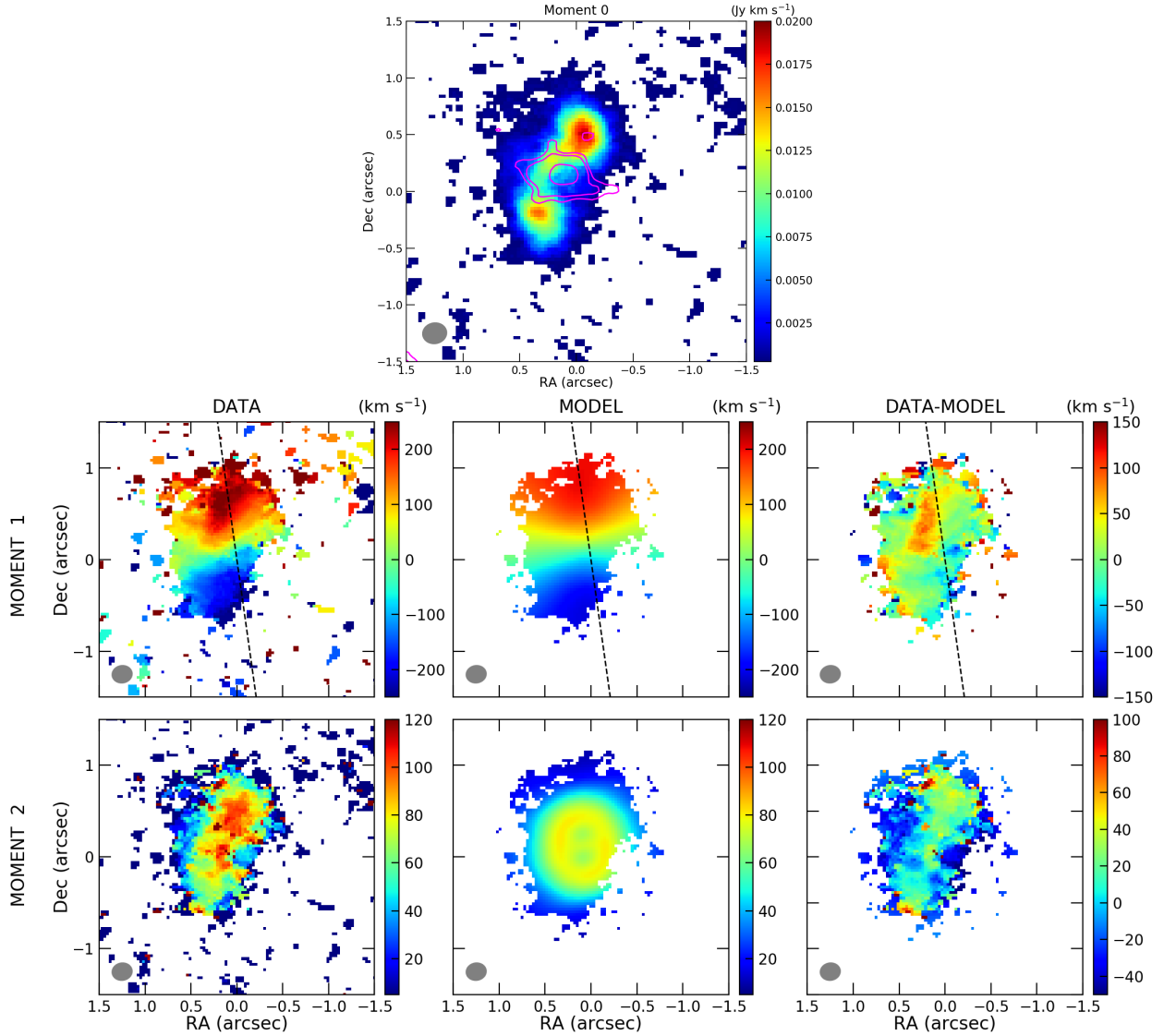
Fig. 11. Same as in Fig. 5 but for J1430. Continuum contours starting at 3\sigma are shown in pink in the moment 0 map ( \sigma = 0.015 mJy beam ^{-1} ), and beam size is 0.21'' \times 0.18'' .
