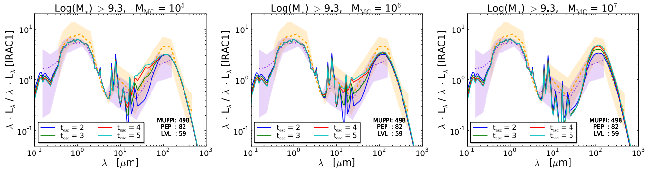
Figure B2. Dependence of SEDs on GRASIL-3D parameters. In all plots, only galaxies with \log(M_*) > 9.3 M_\odot and M_{MC} = 10^5 M_\odot (left), M_{MC} = 10^6 M_\odot (middle), M_{MC} = 10^7 M_\odot (right) are taken into account. In each plot, all the SEDs are normalized to the IRAC1 band (3.6 \mu\text{m} ), continuous colour lines show the median values for different t_{\text{esc}} , while orange and violet dot-dashed lines represent the median value for PEP and LVL samples, respectively, and finally the corresponding filled regions give the 1\sigma uncertainty. Every plot reports the number of galaxies in the MUPPIBOX, PEP and LVL samples.
