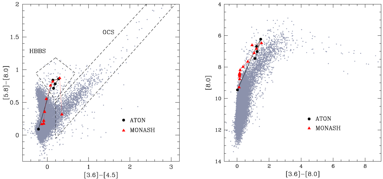
Figure 4. The evolution of the ATON and MONASH models of initial mass 5.5 M_{\odot} and metallicity Z = 8 \times 10^{-3} in the colour-colour ( [3.6] - [4.5] , [5.8] - [8.0] ) plane (left-hand panel) and in the colour-magnitude ( [3.6] - [8.0] , [8.0] ) diagram. The points are taken at time intervals of 3 \times 10^4 yr. Grey dots indicate the sample of AGBs in the LMC by Riebel et al. (2012). The two boxes enclose the regions of the colour-colour plane where OCS and oxygen-rich stars (HBBS) are expected to evolve, based on the present analysis and on the works by Dell’Agli et al. (2014b, 2015).
