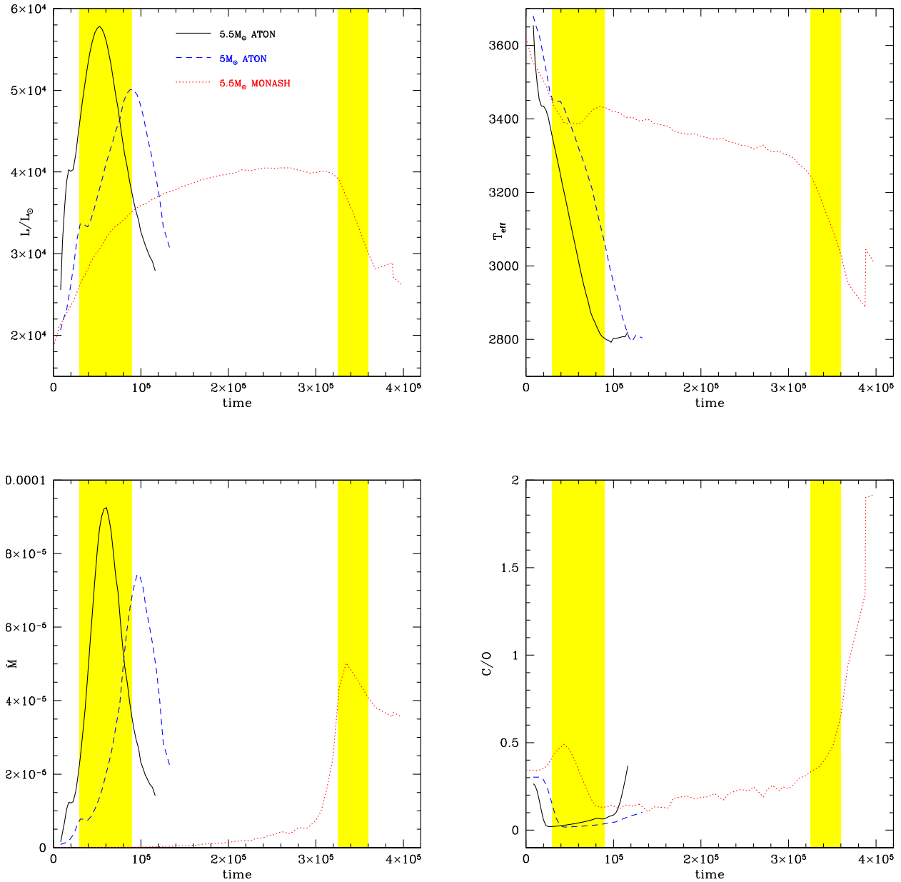
Figure 1. The evolution of luminosity (left-top panel), effective temperature (right-top), mass-loss rate (left-bottom) and surface C/O ratio (right-bottom) of massive AGB models calculated with the ATON and MONASH stellar evolution codes. Times are counted from the beginning of the AGB phase. The shaded regions indicate the phase of highest mass-loss rate and strongest infrared emission for the ATON and MONASH models of initial mass 5.5 M_{\odot} .
