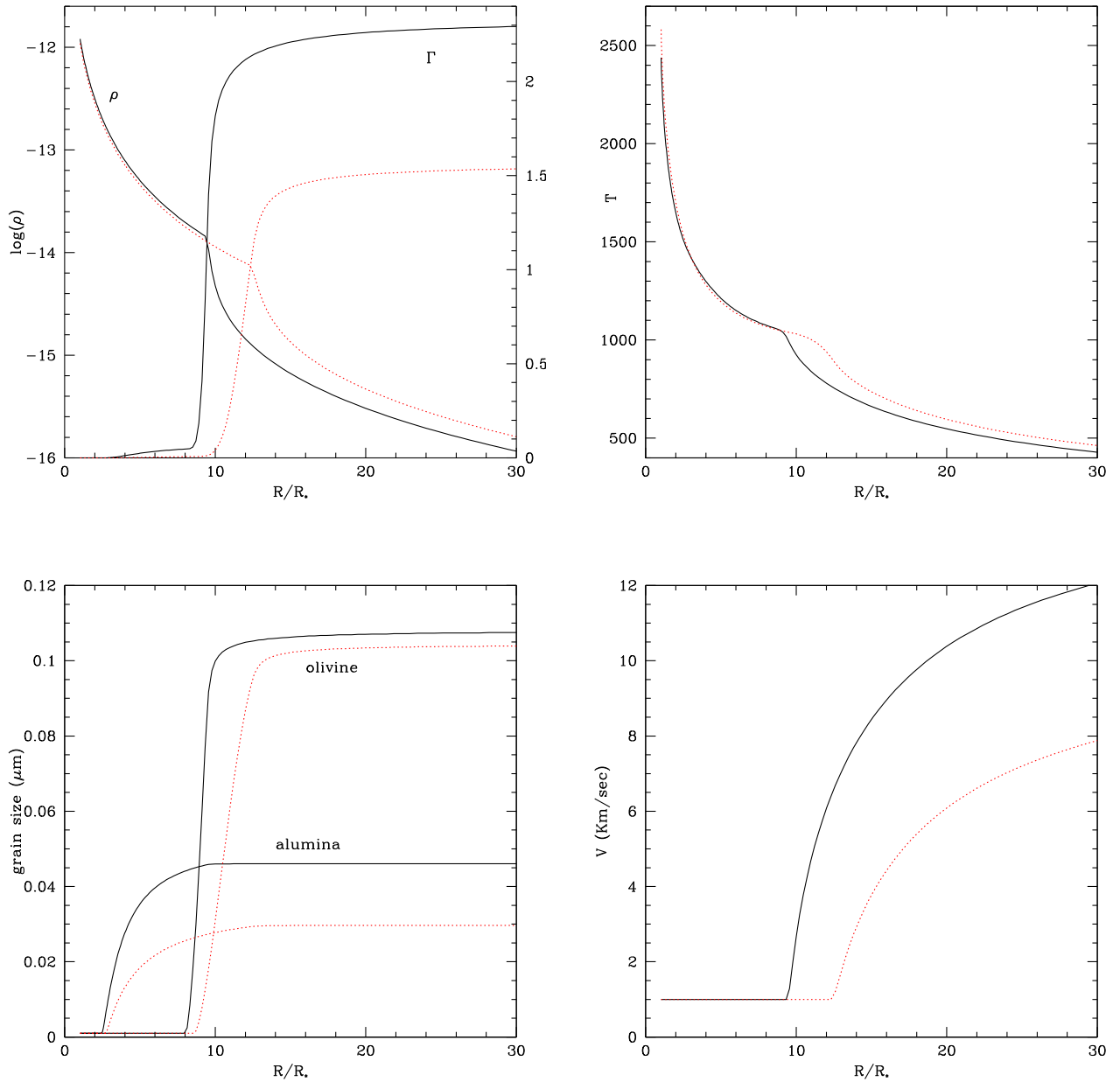
Figure 3. The structure of the wind of the ATON (solid) and MONASH (dotted) models during the phase of highest mass-loss rate. The quantities shown are the radial profiles of density and \Gamma (left-top panel), temperature (right-top), size of the grains formed (left-bottom) and velocity of gas (right-bottom). Distances are measured from the centre of the star and are expressed in units of stellar radii.
