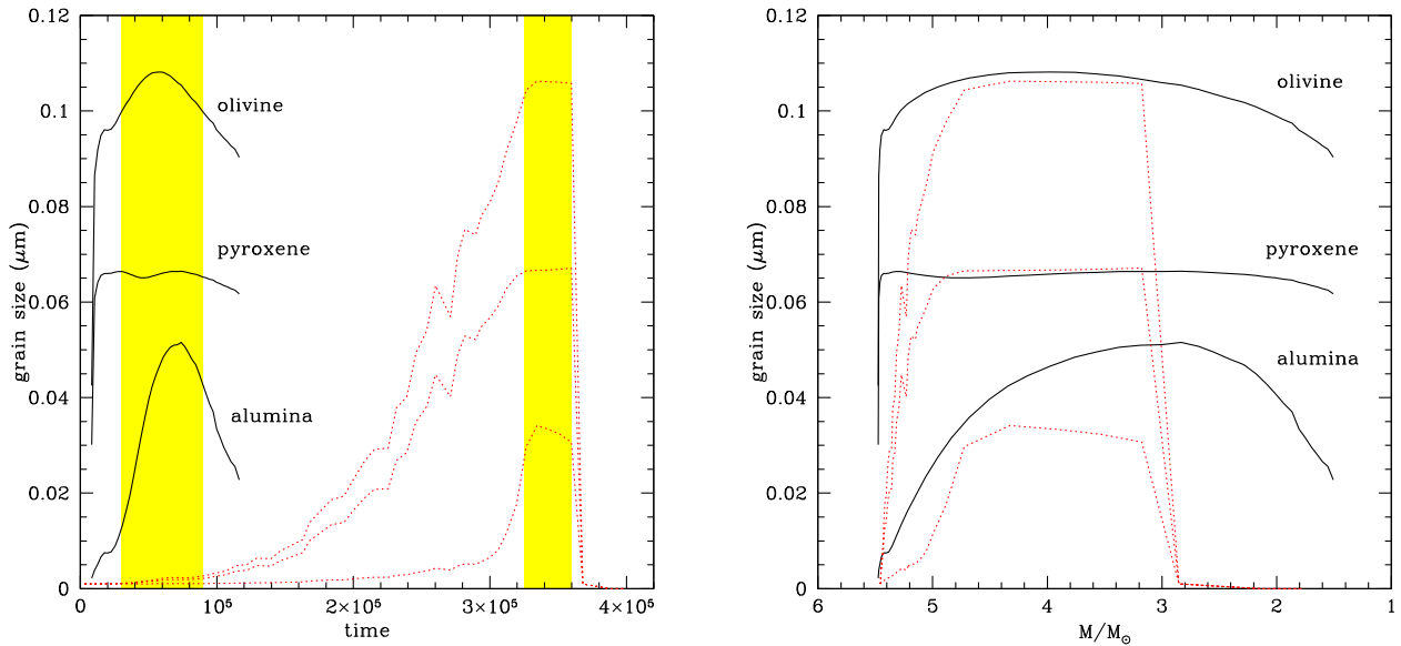
Figure 2. Evolution of the size of the olivine, pyroxene and alumina dust grains formed in the wind of the 5.5 M_{\odot} models shown in Fig. 1 during the AGB phase. The variation of the grain size as a function of the time counted from the beginning of the AGB phase (left-hand panel) and of the current mass of the star (right-hand panel) are shown. The two sets of tracks indicate results from ATON (solid) and MONASH (dotted) codes. The shaded regions in the left-hand panel have the same meaning as in Fig. 1.
