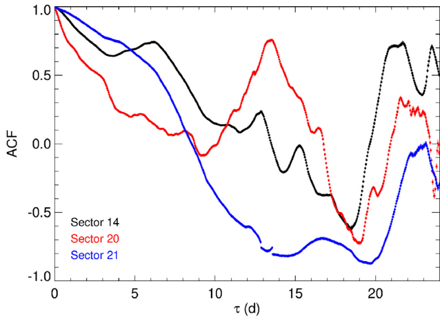
Figure 10. Autocorrelation function of the TESS light curve in Sector 14 (black), Sector 20 (red), and Sector 21 (blue). The ACF is binned in 1 h time lag intervals.
