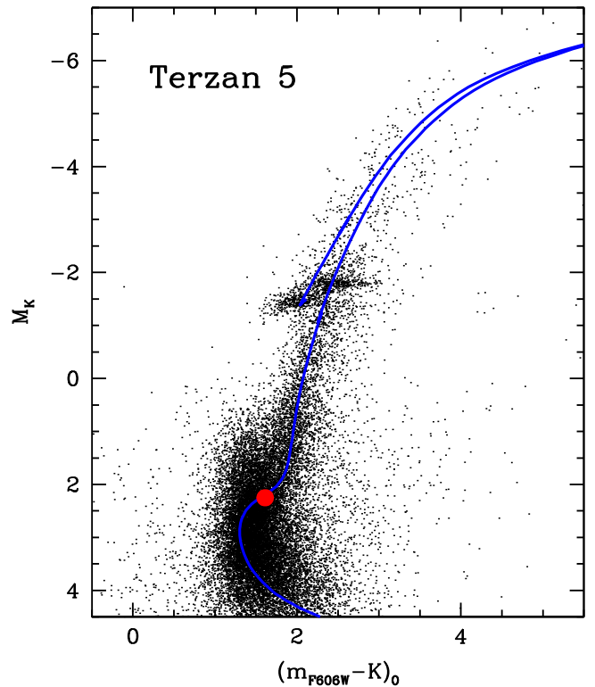
Figure 4. Absolute ( M_K , m_{F606W} - K ) 0 CMD of Terzan 5 obtained from a combination of HST /ACS and ESO/MAD observations. The position of COM-EXO 1745-248 in the quiescent state is marked with the large red circle. The blue line corresponds to a 12 Gyr isochrone with [\text{Fe}/\text{H}] = -0.3 (from Girardi et al. 2010), well reproducing the main metal-poor sub-population of Terzan 5.
