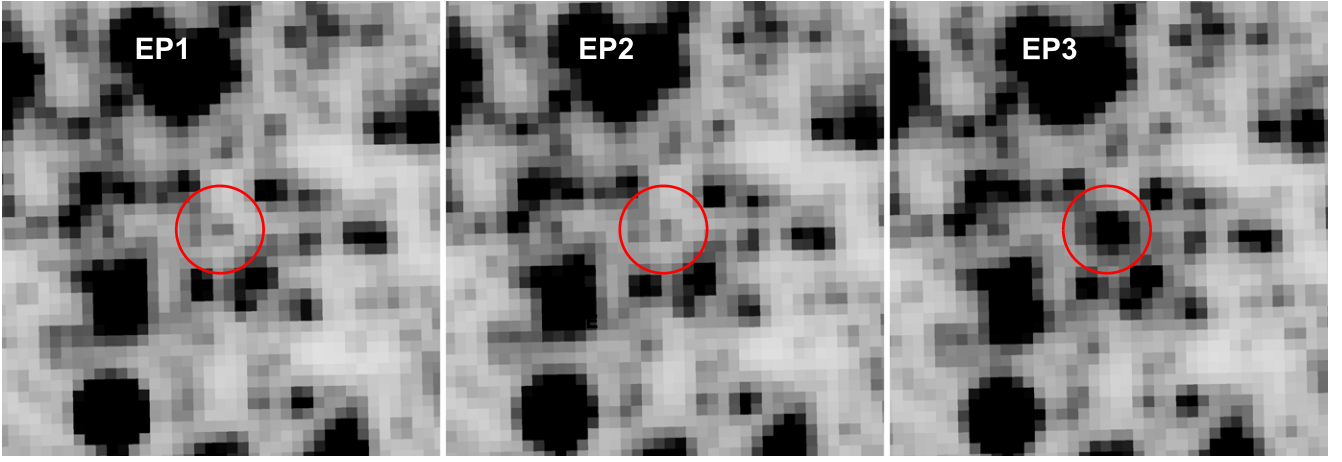
Figure 1. HST /ACS drz combined images of the 2'' \times 2'' region around EXO 1745-248, in the F814W filter, for the three epochs (EP1, EP2, EP3, from left to right, respectively). The source (highlighted with a red circle) is visible as a faint star during the quiescent epochs EP1 and EP2, while it is observed in an outburst stage during EP3. North is up; east is to the left.
