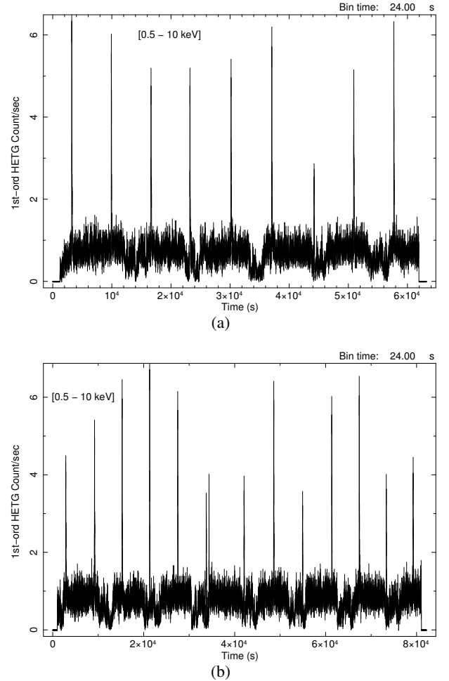
Fig. 2. 1st order background subtracted Chandra /HETG light curves of the observations 14377 a) and 13721 b) in the energy range 0.5–10 keV. The light curve a) starts on 19 December 2011 at 01:03:10 UT, while the light curve b) starts on 23 December 2011 at 20:11:09 UT. The bin time is of 24 s.
