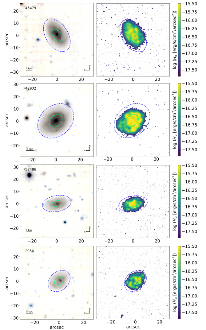
Figure 3. Same as Fig. 2, but for four galaxies representative of the GASP control sample. In these galaxies H\alpha extends at most to 3r_e and the galaxy boundaries are not jagged.
