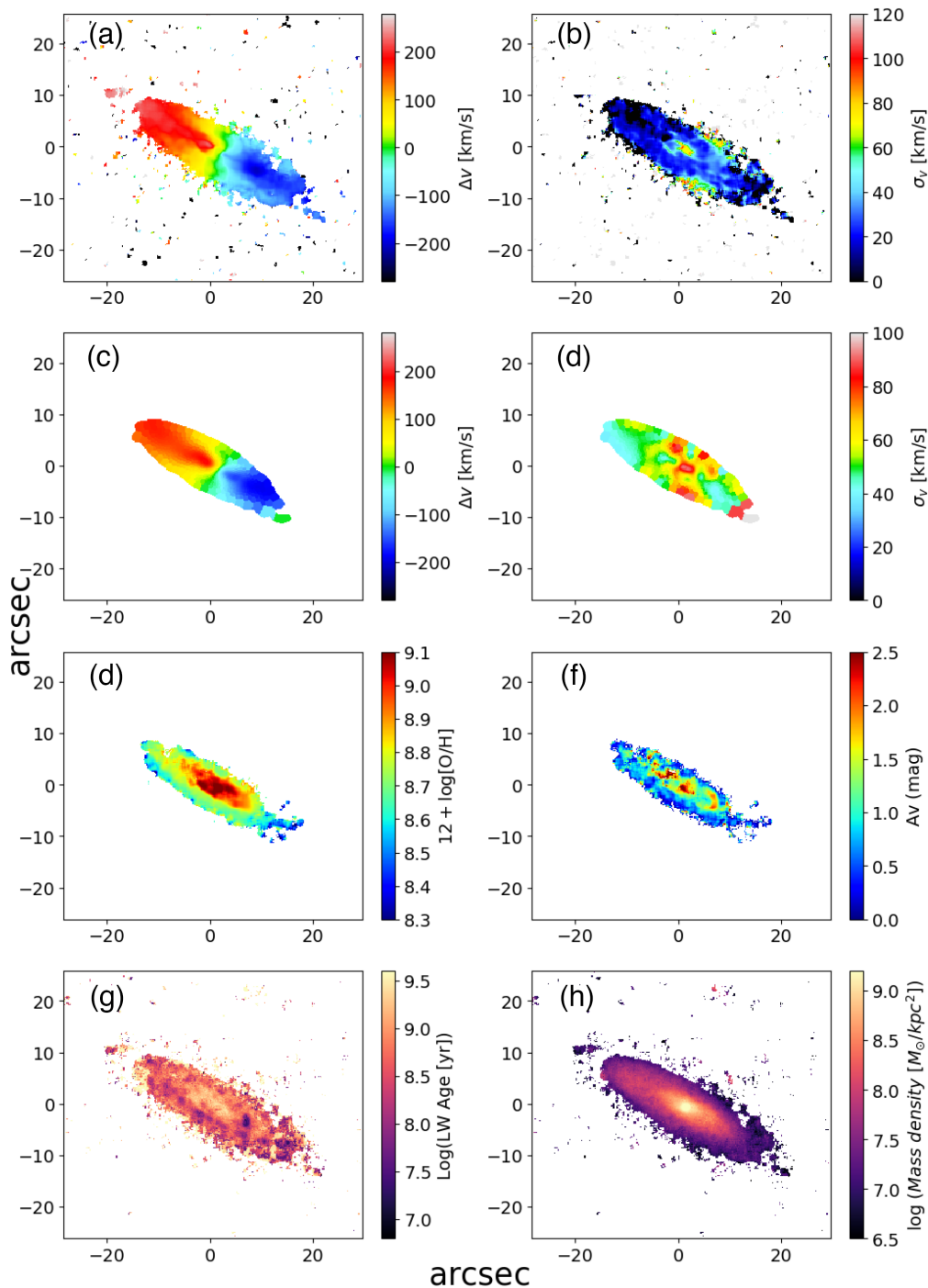
Figure 8. P8721. Panels are as in Fig. 5.
