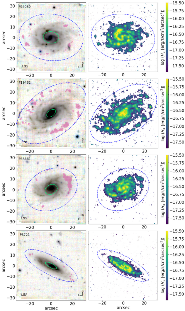
Figure 2. RGB (left) and H\alpha (right) images of the targets. From top to bottom P90580, P19482, P63661, and P8721 are shown. The reconstructed g , r , i filters from the MUSE cube have been used. North is up, and east is left. Colour map is inverted for display purposes. In all the plots, the green ellipses show the r_e , the dashed blue ellipses show the maximum radius at which H\alpha is detected (see text for details). Purple areas show the detached clouds (see text for details). Asymmetries in the star and gas distributions are seen in all galaxies, with one side of the galaxies extending more than the other. All these galaxies have H\alpha extending beyond 4r_e and show patchy H\alpha distribution.
