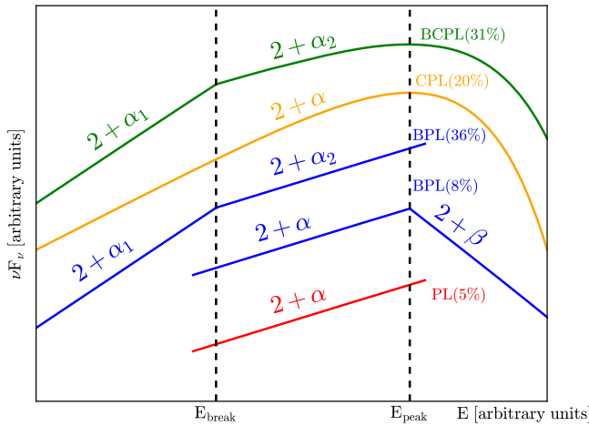
Figure 2. Summary of the four spectral models adopted in this work, and definition of the adopted notation for the spectral indices and characteristic energies. Each one of the analyzed spectra is well described by one of these models. From top to bottom: a broken power law with a high-energy exponential cutoff (BCPL; green), a cutoff power law (CPL; orange), a broken power law (BPL; blue), and a single power law (PL; red). For the BPL model, we found two different cases in our analysis: both indices are larger than -2 (in this case they are called \alpha_1 and \alpha_2 ), or the first index is >-2 and the second one is <-2 (in this case they are called \alpha and \beta , respectively). The percentages quoted next to each model name refer to time-resolved analysis for periods where XRT data are available.
