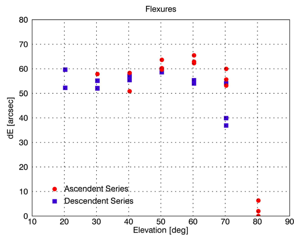
Figure 13: Flexures measured for a chosen azimuthal position for elevation angles between 20^\circ and 80^\circ .
