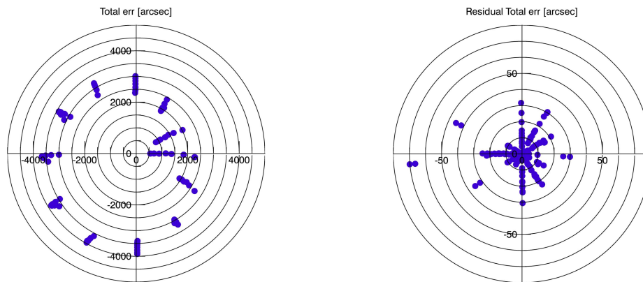
Figure 15: Total error on the sky before model (left) and after the fit (right). The quite important azimuth tilt is evident in the left panel.
