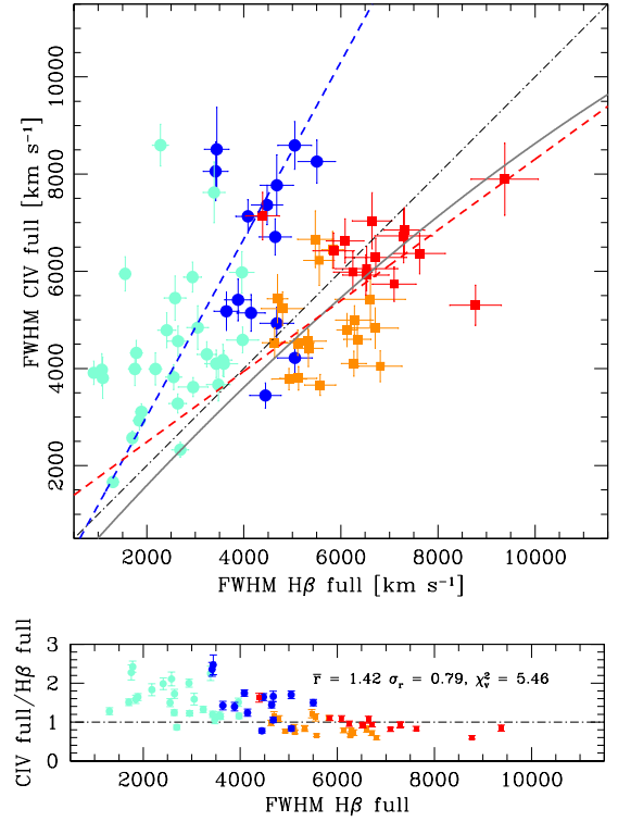
Fig. 3. Top panel: FWHM(Civ\lambda 1549) vs. FWHM(H\beta) (full profiles) for the FOS+HE sample. Data points are color-coded according to sample and population: HE Pop. A – blue circles (●), HE Pop. B – red squares (■), FOS Pop. A – aquamarine circles (●), and FOS Pop. B – golden squares (■). Best fitting least-square lines (dashed) are shown in blue for all Pop. A and red for all Pop. B. The black dot-dashed line is the equality line. The continuous gray line is the expected FWHM following the correction of Sulentic et al. (2006a, corr) . Lower panel: ratio between FWHM Civ\lambda 1549 and FWHM H\beta as a function of FWHM(H\beta) .
