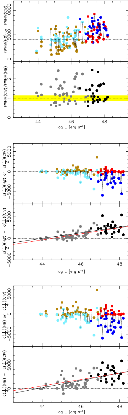
Fig. 9. H\beta and C\text{IV}\lambda 1549 profile parameter comparison as a function of luminosity. Top panels: behavior of \text{FWHM } C\text{IV}\lambda 1549 and H\beta (upper half) and of the ratio \text{FWHM}(C\text{IV}\lambda 1549)/\text{FWHM}(H\beta) as a function of L (lower half), for FOS (golden and pale blue) and HE sample (red and blue). The yellow band identifies the region where \text{FWHM}(C\text{IV}\lambda 1549)/\text{FWHM}(H\beta) = 1 within the errors. Middle panels: c(\frac{1}{2}) of H\beta and C\text{IV}\lambda 1549 (upper half), and difference \delta(\frac{1}{2}) as a function of L (lower half). Square symbols indicate Pop. B, circles Pop. A. Lines trace an unweighted least-squares fit for the Pop. A (black) and for Pop. B (red) sources. Bottom panels: as in top panels but for c(\frac{1}{4}) and \delta(\frac{1}{4}) . The vertical dotted lines join H\beta and C\text{IV}\lambda 1549 parameters for the same object (e.g., they are not error bars).
