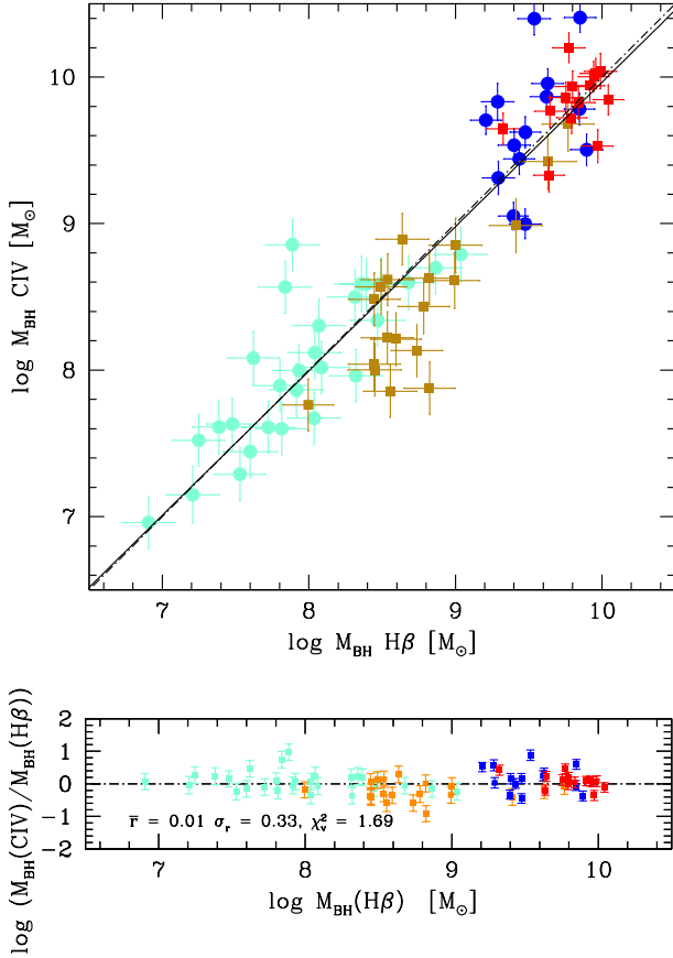
Fig. 12. M_{\text{BH}} computed from the fiducial relation of Vestergaard & Peterson (2006) based on FWHM H \beta vs. the one computed from the C \lambda 1549 FWHM corrected following Eq. (6). Error bars include luminosity uncertainties estimated by the scatter in L derived from the UV and the visual spectral ranges along with errors on FWHM propagated quadratically. Lower panel: residuals for the three cases. Meaning of the color-code is the same as in the previous Figs.
