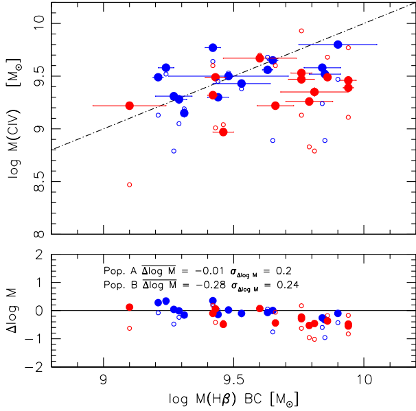
Fig. 8. Black hole mass computed from the fiducial relation of Vestergaard & Peterson (2006) based on FWHM H \beta vs. the ones computed from the C iv \lambda 1549 FWHM following Park et al. (2013), for Pop. A (blue) and B (red) HE sources. Values of M_{\text{BH}} obtained from the Vestergaard & Peterson (2006) C iv \lambda 1549 scaling law after the correction suggested by Brotherton et al. (2015, small dots) are shown by small open circles. Lower panel: residuals as a function of M_{\text{BH}} . The average and the scatter reported for Populations A and B refer to the Park et al. (2013) scaling laws.
