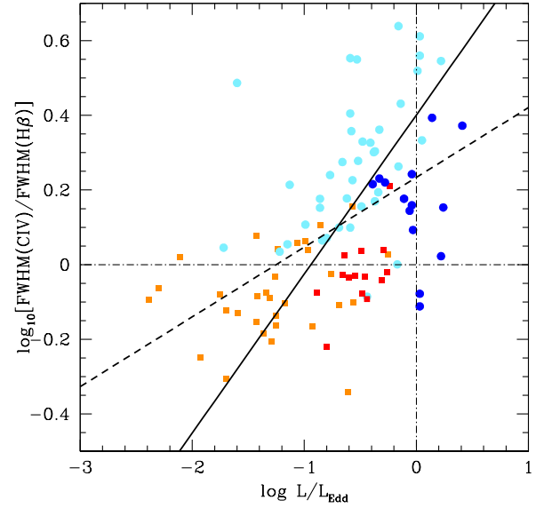
Fig. 4. Relation between the logarithm of the FWHM ratio of C IV \lambda 1549 to H \beta and the logarithm of the Eddington ratio L/L_{\text{Edd}} . The vertical dot-dashed line traces the Eddington limit. The colors and shapes of symbols are as in Fig. 3. The dashed line is an unweighted least-squares fit, and the filled line was obtained with the bisector method (Feigelson & Babu 1992).
