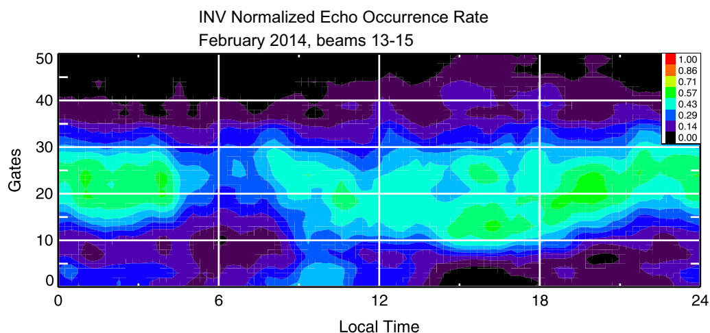
Fig. 2 A contour plot of the echo occurrence rate versus local time for the Inuvik radar in beams 13–15 and gates 0–50. Solar local time was counted for the radar location, LT = UT - 7 . Data at all radar operating frequencies were considered
