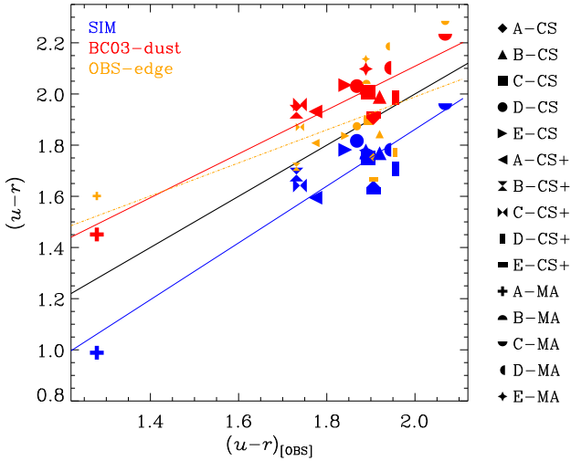
Figure 3. (u-r) colours of the simulated galaxies using the SIM, BC03-dust and OBS-edge methods, as a function of the corresponding values obtained with OBS. We also show the one-to-one relation (black line) and linear fits of SIM, BC03-dust and OBS-edge (blue, red and orange lines, respectively).
