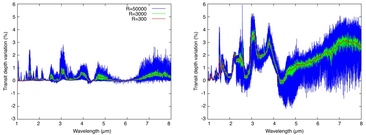
Figure 5. Difference spectra in percent between the model with L_X = 10^{28} and 10^{26} \text{ erg s}^{-1} (left panel) and the model with L_X = 10^{30} and 10^{26} \text{ erg s}^{-1} (right panel), constructed using three values of the resolving power, R = 300 (red line), 3000 (green line), and 50,000 (blue line).
