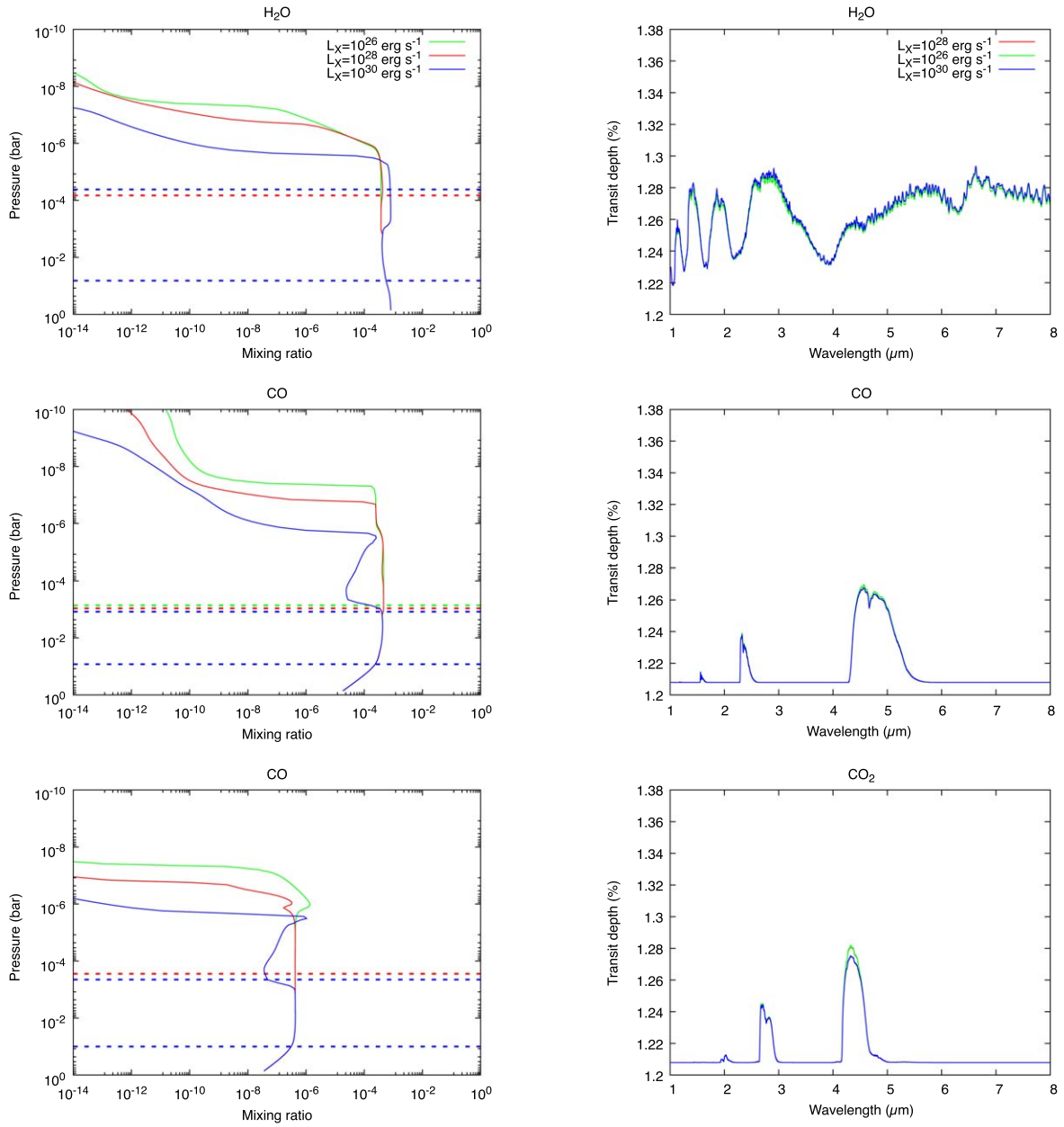
Figure 4. Same as Figure 3 for the negatively reacting species, \text{H}_2\text{O} , \text{CO} , and \text{CO}_2 .
