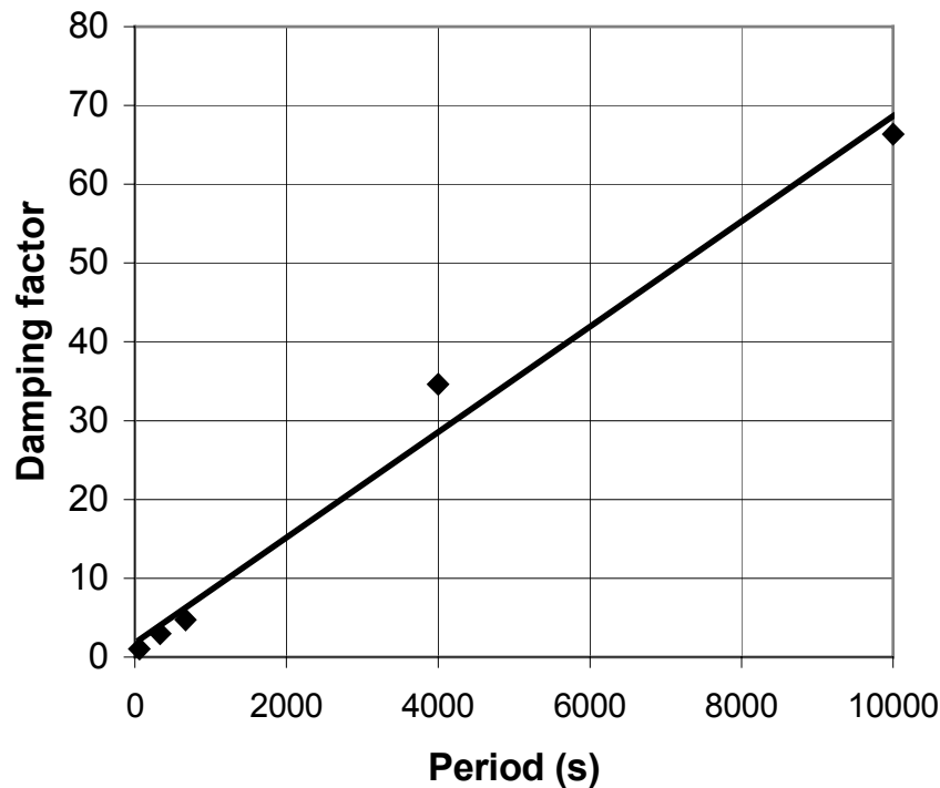
Figure 5-1 – Destriping damping factor for periodic oscillations versus \tau_f (the period of the fluctuation). Dots indicate the values obtained from maps while the solid line represents a linear interpolation.
