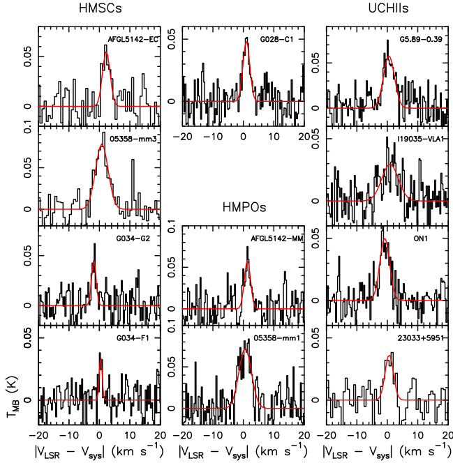
Figure 1. Spectra of the \text{HOCO}^+ ( 4_{0,4} - 3_{0,3} ) line in the 11 detected sources. The y-axis is in T_{\text{MB}} units. The x-axis corresponds to |V_{\text{LSR}} - V_{\text{sys}}| , i.e. the difference between the local standard of rest velocity, V_{\text{LSR}} , and the nominal systemic velocity, V_{\text{sys}} , given in Fontani et al. 2011. The red curves superimposed on the spectra represent the best gaussian fits.
