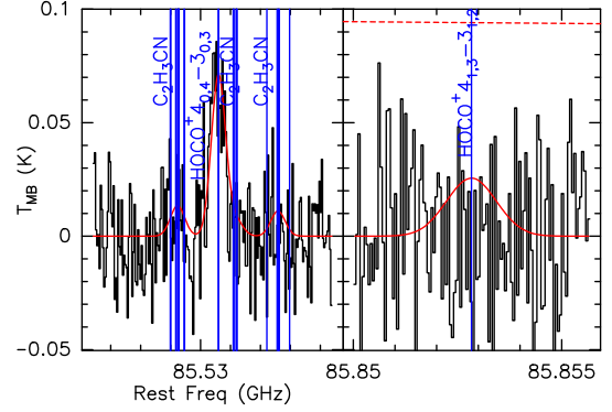
Figure 2. Left panel: spectrum of the \text{HOCO}^+ 4_{0,4} - 3_{0,3} line towards 05358-mm1 superimposed on the synthetic spectrum (in red) calculated with MADCUBA. The synthetic spectrum is calculated for a \text{HOCO}^+ column density of 4.3 \times 10^{12} \text{ cm}^{-2} and a \text{C}_2\text{H}_3\text{CN} column density of 10^{18} \text{ cm}^{-2} , which is the value measured towards Sgr B2(N) (see Sect. 3). The rest frequencies of the nearby \text{C}_2\text{H}_3\text{CN} transitions are indicated by vertical lines. Right panel: spectrum of 05358-mm1 centred on the rest frequency of \text{HOCO}^+ 4_{1,3} - 3_{1,2} , superimposed on the synthetic spectrum created with the same parameters used in Left panel: the expected peak of the line is well under the 3\sigma rms noise (shown by the red dashed horizontal line).
