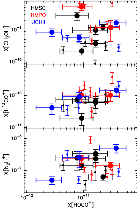
Figure 3. Abundance of \text{HOCO}^+ against that of, from top to bottom: \text{CH}_3\text{OH} , \text{H}^{13}\text{CO}^+ , and \text{N}_2\text{H}^+ . The colours indicate the different evolutionary groups as labelled in the top-left corner. The large filled symbols correspond to the detected sources, while the small triangles indicate the upper limits on the abundance of \text{HOCO}^+ . In the panel with \text{X}[\text{H}^{13}\text{CO}^+] , we do not show 05358-mm3, observed and detected in \text{CH}_3\text{OH} , \text{N}_2\text{H}^+ and \text{HOCO}^+ but not in \text{H}^{13}\text{CO}^+ .
