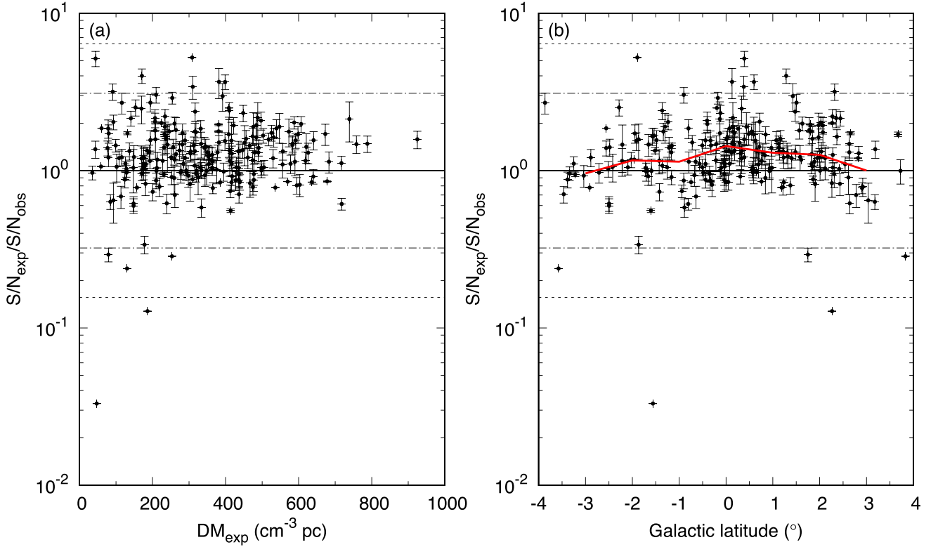
Figure 1. A comparison of the expected versus observed S/N values ( S/N_{\text{exp}} and S/N_{\text{obs}} , respectively) for pulsars redetected in 44 per cent of the HTRU-S LowLat survey. Panel (a) shows S/N_{\text{exp}}/S/N_{\text{obs}} plotted against the PSRCAT DM for each redetected pulsar, while panel (b) shows S/N_{\text{exp}}/S/N_{\text{obs}} plotted as a function of each pulsar’s Galactic latitude. The bold line in each case represents the 1:1 relation, while the surrounding dashed lines extending outwards from the 1:1 line indicate contours containing 95 per cent and 99 per cent of the redetections, respectively. The red line in panel (b) shows the median of the scatter, determined using bins with a width of 1^\circ .
