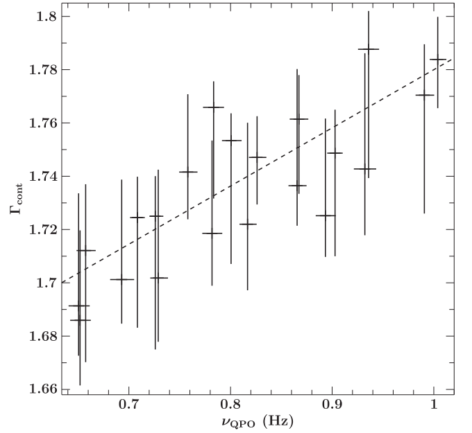
Figure 7. Correlation between the best-fit QPO frequency \nu_{\text{QPO}} and the photon index of the power-law continuum \Gamma_{\text{cont}} from model 4. Superimposed is the best-fit linear correlation with a slope of 0.22 \pm 0.11 .
