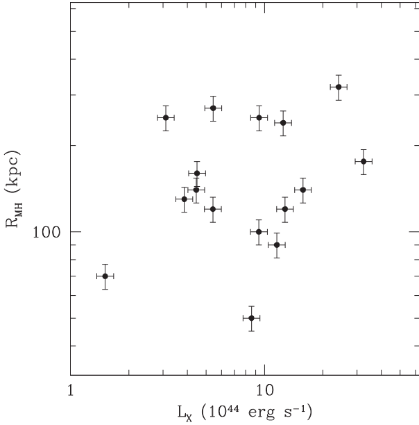
Fig. 3. Average radius of the mini-halo (from Giacintucci et al. 2014b ; Bravi et al. 2016 ) versus the X-ray luminosity inside R_{500} (taken from Piffaretti et al. 2011 , and converted into the 0.5–2.0 keV band). No obvious correlation is visible (we found r_s \sim 0.2 , with a probability of no correlation of probs \sim 40\% ).
