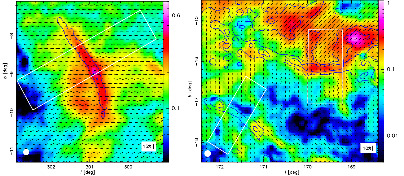
Fig. 7. Observed polarized emission at 353 GHz (in MJy sr -1 ) of the Musca ( left ) and Taurus ( right ) clouds. The maps are at the resolution of 9.6 (indicated by the white filled circles) for increased S/N. The black segments show the \mathbf{B}_{\text{POS}} -field orientation ( \psi+90^\circ ). The length of the pseudo-vectors is proportional to the polarization fraction. The blue contours show the total dust intensity at levels of 3 and 6 MJy sr -1 , at the resolution of 4.8. The white boxes correspond to the area of the filaments and their backgrounds that is analysed in the rest of the paper.
