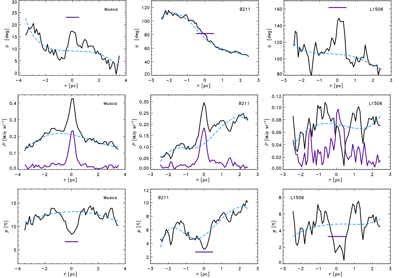
Fig. 10. Observed profiles (in black) of the polarization angle, the polarized intensity, and the polarization fraction, from top to bottom . The dashed blue curves show the variation of the background values of \psi_{\text{bg}} , P_{\text{bg}} , and p_{\text{bg}} derived from I_{\text{bg}} , Q_{\text{bg}} , and U_{\text{bg}} . On the middle three plots , the P_{\text{fil}} profiles in purple are derived from the polynomial fits I_{\text{fil}} , Q_{\text{fil}} , and U_{\text{fil}} . On the top and bottom plots , the horizontal purple lines indicate the mean values of the intrinsic polarization angle and fraction of the filaments for |r| \leq R_{\text{out}} .
