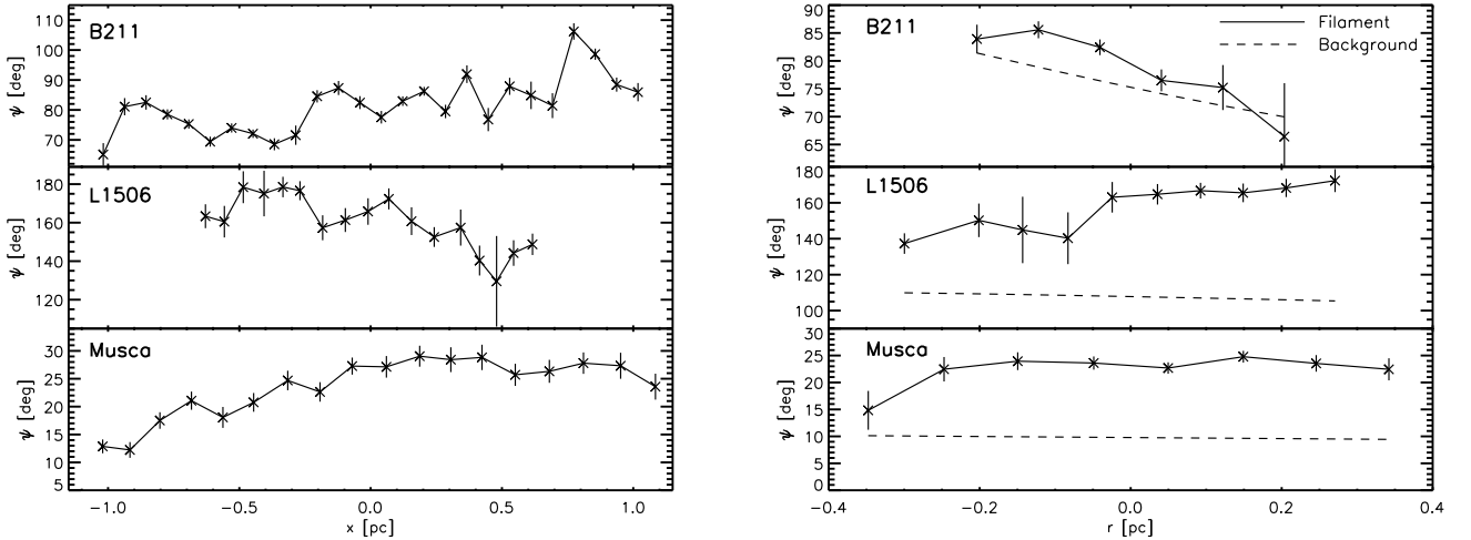
Fig. 11. Filament intrinsic polarization angle along (left panel), and perpendicular (right panel) to, the crests of the filaments. The crosses are data points computed from Q and U values, after averaging the background subtracted maps in the direction perpendicular (left panel) and parallel (right) to the filament crests. In the left panel, x is a coordinate along the filament crest, while in the right panel, r is the radial distance to the filament crests. In the right panel, the dashed line represents the background polarization angle. The beam is 0.3 pc for Musca, and 0.2 pc for B211 and L1506.
