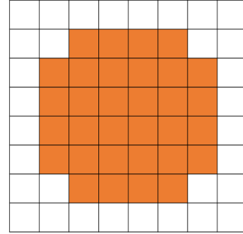
Figure 3. Simplified schematic of the 8 \times 8 array of antennas to be placed at the focal plane of a large radio telescope. Each element will be sensitive to two orthogonal linear polarization signals. The inner 32 antenna elements (in orange) are active, i.e. cascaded with MMIC LNAs. The outer elements (in white) are dummy.
