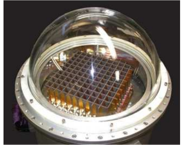
Figure 1. C-band PHAROS array showing the 10×11 dual polarization Vivaldi antennas through half-dome Plexiglas vacuum window.
