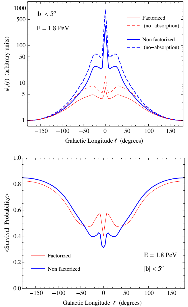
FIG. 14. Top panel: Longitude distribution of the gamma-ray flux at E = 1.8 PeV, integrated in the latitude range |b| < 5^\circ . The flux is shown for both our models (factorized and nonfactorized emissions), including and neglecting the effects of absorption. Bottom panel: Average survival probability for gamma rays of energy E = 1.8 PeV, averaged in the latitude interval |b| < 5^\circ , as a function of the Galactic longitude, according to our two models.
