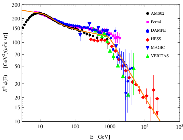
FIG. 3. Flux of electrons plus positrons observed at the Earth. The line is our fit to the spectrum. The data points are from Fermi [39], AMS02 [40], DAMPE [46], HESS [41–43], MAGIC [44] and VERITAS [45].
