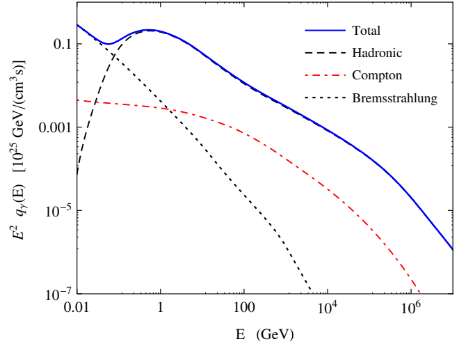
FIG. 4. Gamma-ray emission rate in the solar neighborhood. The total emission and the single contributions of the three main mechanisms (hadronic, bremsstrahlung and Compton scattering) are shown. The assumed hydrogen density in the interstellar medium is n = 1 \text{ cm}^{-3} .
