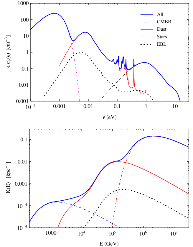
FIG. 1. Top panel: Energy distribution of soft photons in the solar neighborhood. Bottom panel: Absorption coefficient K(E, \vec{x}_{\odot}) (averaged over the direction of the photon) for gamma rays in the solar neighborhood, plotted as a function of the gamma-ray energy E . In both panels the curves are given for the total and for the contributions of each component of the target radiation field.
