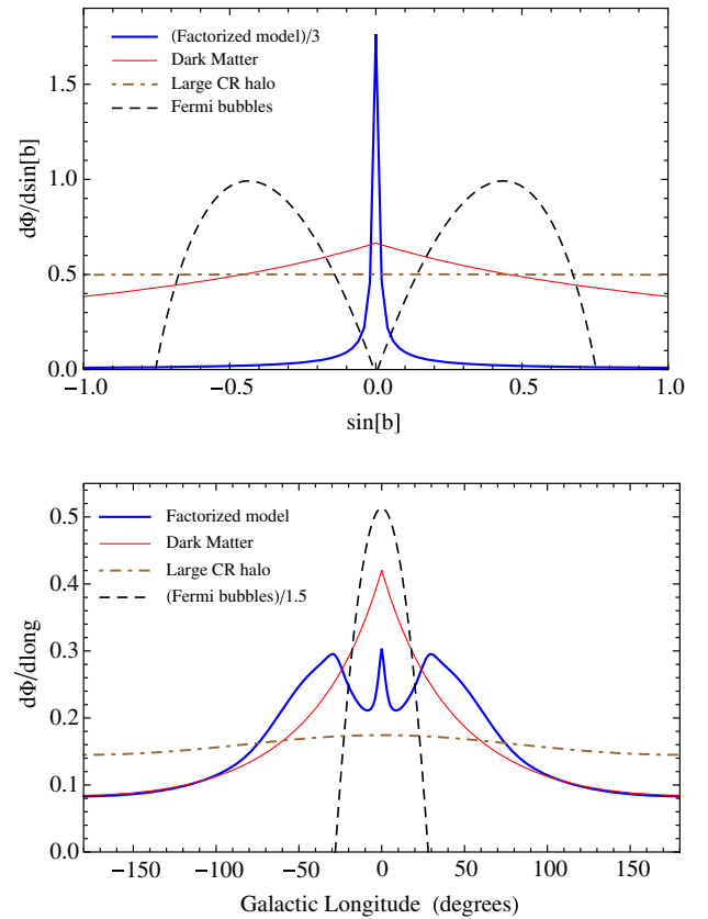
FIG. 17. Angular distributions of the Galactic gamma-ray flux for different emission models: Galactic model with factorized emission, dark matter decay model [61,62], large CR halo model [64] and emission from the Fermi bubbles [65]. Top panel: Latitude ( \sin b ) distributions. Bottom panel: Longitude distributions. The curves are calculated neglecting the absorption effects and are normalized to unit area (except where noted).
