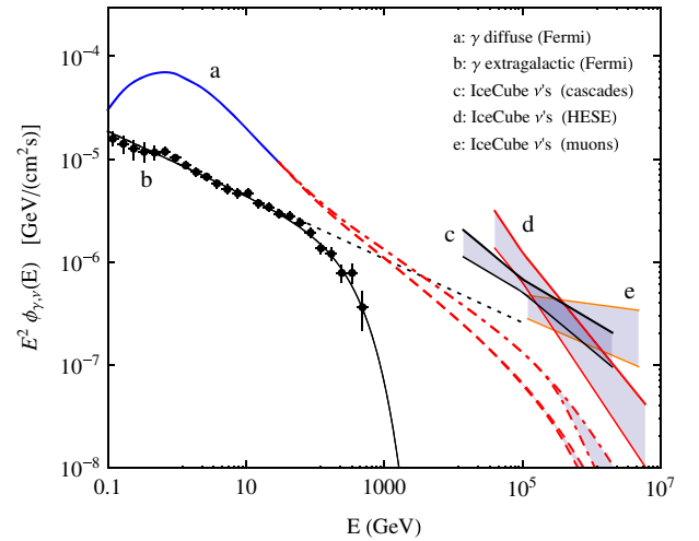
FIG. 16. Curve a shows the diffuse Galactic gamma-ray flux observed by Fermi (solid line) and the extrapolations calculated under the assumptions of a factorized (dashed line) and nonfactorized (dot-dashed line) emission. The Fermi measurement of the extragalactic gamma-ray flux [58] is shown by data points and with line (b) that is a fit with the functional form of a power law with an exponential cutoff (the dashed line shows the fit extrapolation without the cutoff). The shaded regions c , d and e show estimates of the neutrino flux obtained by IceCube under the assumption of an isotropic extragalactic flux [19]. All fluxes are integrated over the entire sky.
