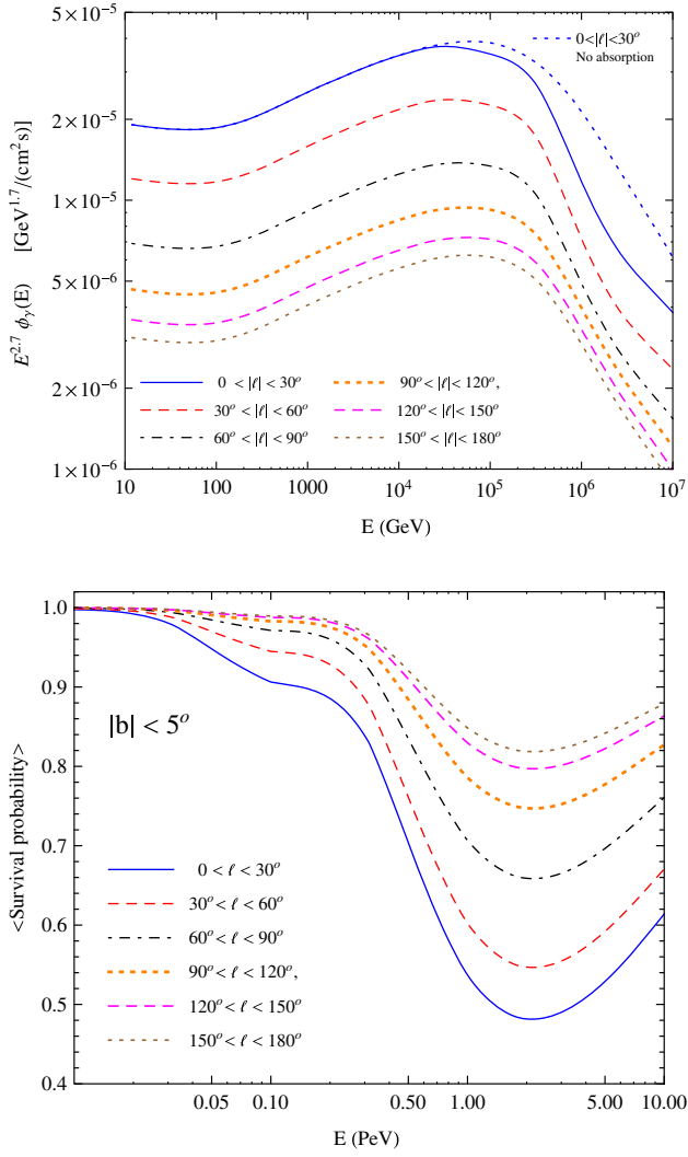
FIG. 9. Top panel: Gamma-ray flux as a function of energy, according to the model where the emission is factorized. The flux is integrated in latitude in the range |b| < 5^\circ and in six longitude intervals. From top to bottom: |l| < 30^\circ , 30^\circ < |l| < 60^\circ , 60^\circ < |l| < 90^\circ , 90^\circ < |l| < 120^\circ , 120^\circ < |l| < 150^\circ and 150^\circ < |l| < 180^\circ . Absorption effects are included. For the region |l| < 30^\circ the flux calculated neglecting absorption is also reported (as a dotted line). Bottom panel: Average survival probability of gamma rays in the same six angular regions.
