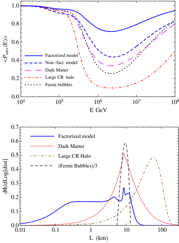
FIG. 18. Top panel: Average survival probability of gamma rays (after integration over the entire sky) for different emission models. Bottom panel: Distribution of the gamma-ray path length for the same models. The distributions are calculated after integration over the entire solid angle, neglecting the effects of absorption, and are normalized to unity (or 1/3 for the Fermi bubbles case).
