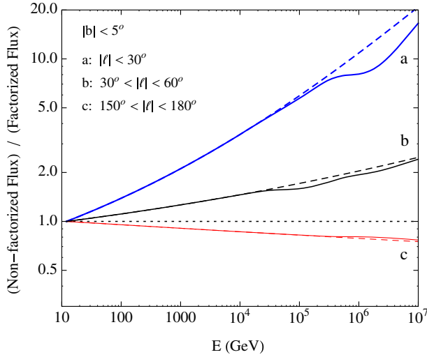
FIG. 13. Ratio between the gamma-ray fluxes calculated according to the nonfactorized and the factorized emission models. The ratio is shown as a function of the gamma-ray energy, after integration in different longitude regions, for the latitude |b| < 5^\circ . The solid (dashed) lines include (neglect) the effects of absorption.
