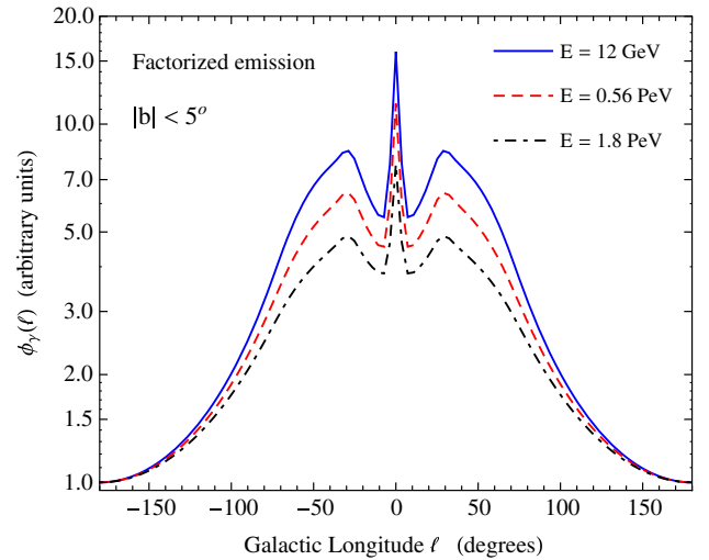
FIG. 10. Longitude distribution of the gamma-ray flux calculated in a model where the emission is factorized. The flux is shown for three values of the energy and it is rescaled to have value unity for l = \pm 180^\circ to make easier a comparison of the shapes of the distributions. The difference in shape for the three distributions is entirely due to energy dependent absorption effects.
