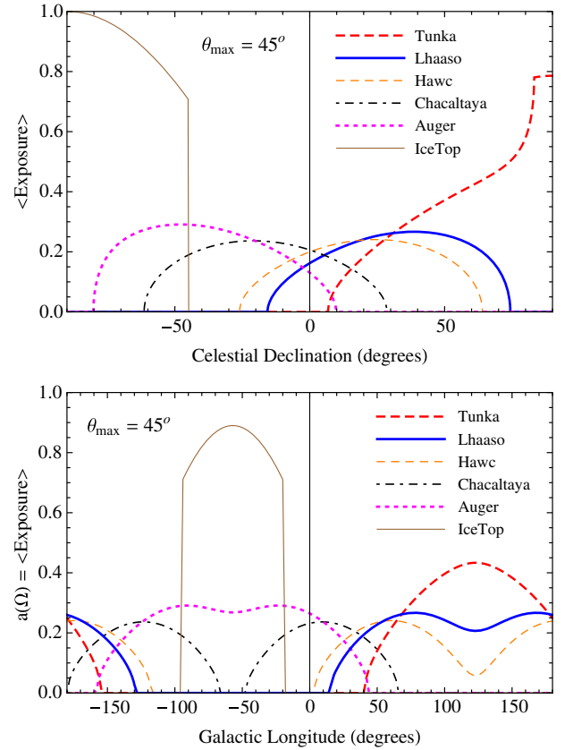
FIG. 21. Top panel: Average exposure for points in the sky with celestial declination \delta . Bottom panel: Average exposure for points on the Galactic equator, as a function of longitude. The exposure is calculated for six detector locations: Tunka ( \lambda = +51.8^\circ ), LHAASO ( \lambda = +29.4^\circ ), HAWC ( \lambda = +19.0^\circ ), Chacaltaya ( \lambda = -16.4^\circ ), Auger ( \lambda = -35.2^\circ ) and IceTop ( \lambda = -90^\circ ).
