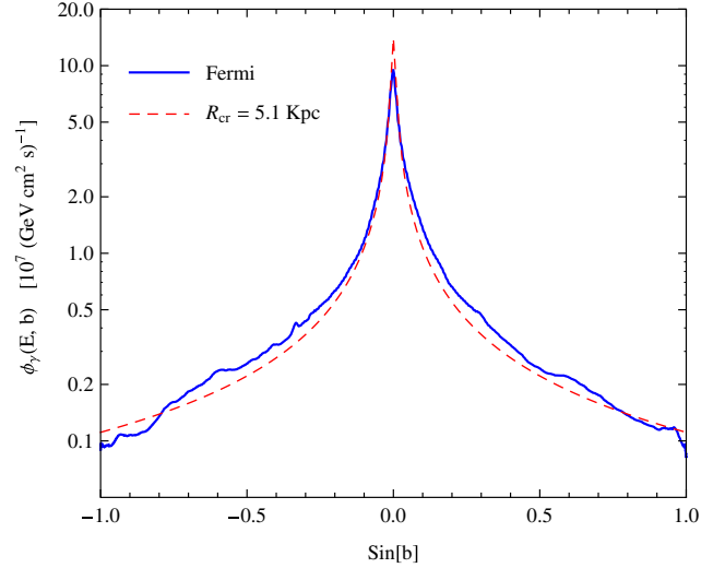
FIG. 8. Latitude distribution of the gamma-ray flux at E^* = 12 GeV according to our model, compared to the Fermi background template.
