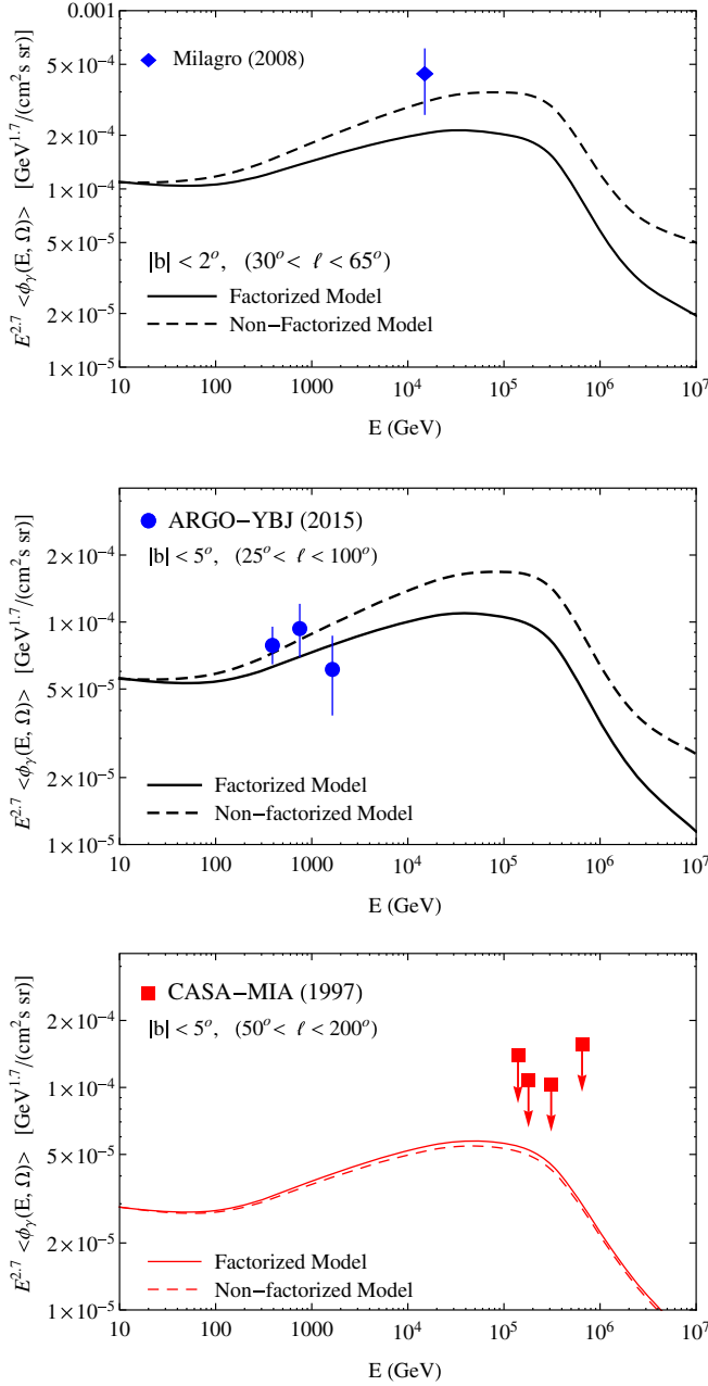
FIG. 20. Measurements of the diffuse gamma-ray flux at high energy, compared to the average flux according to our two models, calculated for the same angular region of the data. The three panels show the measurement of Milagro [8] (top), ARGO-YBJ [9] (middle) and CASA-MIA [14] (bottom).
