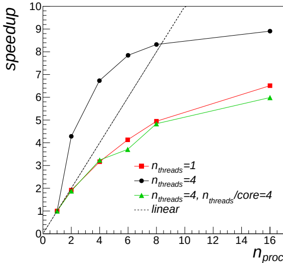
Figure 10. Computational speedup of compact source finding in MPI+OpenMP runs over a 32000 \times 32000 pixel simulated map as a function of the number of allocated MPI processes using n_{threads}=1 (red squares) and n_{threads}=4 (black dots) per MPI process. Green triangles refer to the speedup obtained using n_{threads}=4 per MPI process, with all four threads running on the same computing core rather than in a dedicated core.
