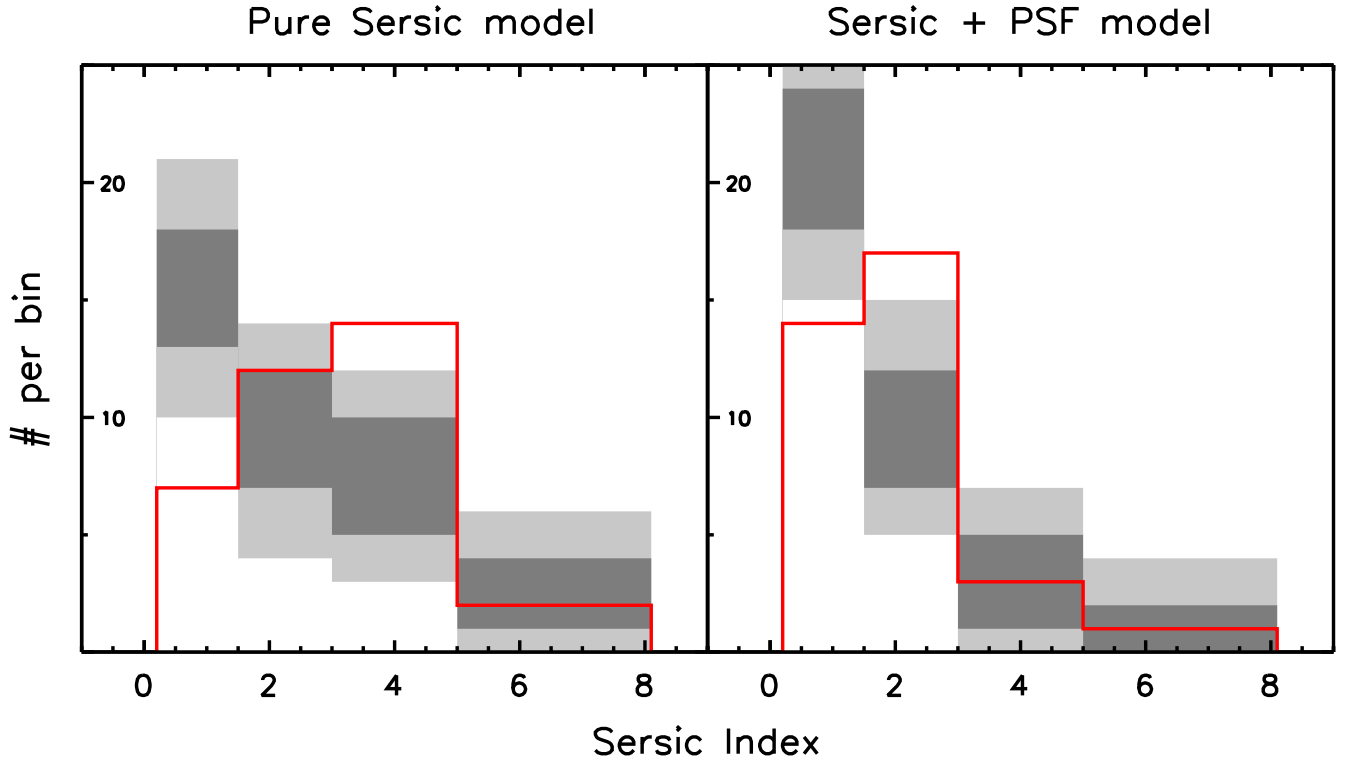
Fig. A.1. Distributions of the Sérsic index ( n ) from GALFIT fits to AGNs and inactive control galaxies in the WFC3/F160W band. 1000 draws of a mass-matched control sample are analysed to determine the 1\sigma/2\sigma scatter in the n distributions for inactive galaxies, shown as dark/light grey zones in the histograms. Red open histograms show the distributions for the AGNs. Left: Results from fits of a single Sérsic elliptical model. Right: Results from fits with two components - a Sérsic elliptical model and a central point source. The inclusion of a point source results in lower Sérsic indices for both AGNs and inactive galaxies.
