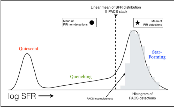
Fig. 12. An illustration useful for understanding Figures 13, 14, 15. The solid curve shows a qualitative schematic SFR distribution of a population of galaxies, for example, massive galaxies at z \sim 2 where SF galaxies outnumber the quiescent population. It is assumed that the L_{60} distribution is identical and tracks the SFR. The measurable L_{60} (or SFR) distribution of galaxies individually detected in the Herschel/PACS maps is shown as a representative grey histogram. At these redshifts, the PEP+GOODS-Herschel PACS catalogs are sensitive to FIR luminosities that trace just deeper than the ridgeline of the SF Sequence (e.g. Rosario et al. 2013b), but the completeness of the catalogs at this limit is low ( \approx 30\% ) leading to a shallow cutoff in the histogram at the faint end. The mean L_{60} of the entire population comes from stacks into the PACS maps (see Section 2.2) and is shown as a dashed vertical line. Since stacking is a purely linear process, the mean is shifted towards the star-forming end in this diagram. Additionally, the mean L_{60} of both PACS detected and undetected galaxies can be determined, shown as a star and circle point as in the later Figures. The schematic also reveals how the fraction of galaxies that are FIR-detected is closely related to the fraction of moderate and strongly SF galaxies in the population.
