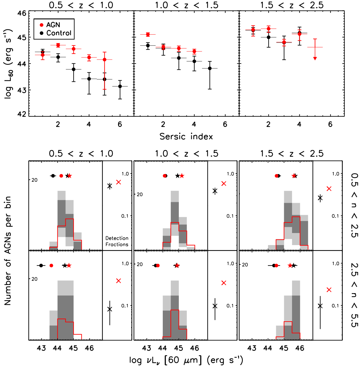
Fig. 13. Mean 60 \mu\text{m} monochromatic luminosities ( L_{60} ) and luminosity distributions of AGNs and inactive control galaxies in both GOODS fields combined, as a function of H-band Sérsic index ( n ). Panels left to right span three distinct bins in redshift. In the top row, the mean L_{60} from combinations of detections and stacks are compared in bins of n . The X-axis error bars show the extent of these bins. The errors on the AGN measurements (red points) are determined from bootstrapping into the AGN subsample in each bin in redshift and n . The errors on the inactive galaxy measurements (black points) come from the analysis of an ensemble of mean L_{60} from 100 random draws of mass-matched control galaxies. In the lower two rows, each panel is split into two subpanels. L_{60} distributions and PACS detection fractions for AGNs and inactive galaxies are plotted in the left subpanels for two coarse bins in Sérsic index. Histograms show the L_{60} distributions of PACS-detected AGNs and inactive galaxies. The 100 random draws of mass-matched control galaxies are used to determine the 1\sigma/2\sigma scatter in L_{60} for inactive galaxies, shown as dark/light grey zones in the histograms. The red histograms are the L_{60} distributions for AGNs. The mean L_{60} corresponding to these histograms are plotted for PACS-detected AGNs as red star points and for inactive galaxies as black star points. Error bars on the latter are the rms scatter of the mean of the control samples. The mean L_{60} of PACS-undetected AGNs (red circle points) and inactive galaxies (black circle points) are also compared similarly. PACS detection fractions are shown in the right subpanels. Red cross points denote AGNs and black cross points denote inactive galaxies, with rms scatter shown as vertical error bars on the latter points. See Section 4.1 for a discussion.
