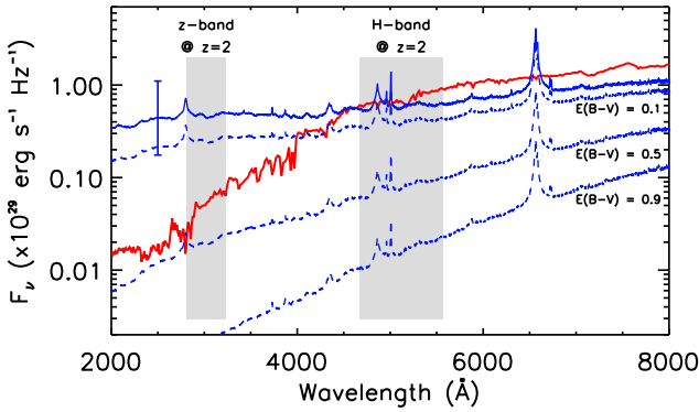
Fig. 8. A comparison of a typical galaxy spectrum (red solid line) and AGN spectra with different levels of extinction (blue lines). The base galaxy spectrum is the ‘Sa’ template from the SWIRE library (Polletta et al. 2007) scaled to correspond to H = 24 magnitude if placed at z = 2 . The base AGN spectrum (blue solid line) is stitched together from composite radio-quiet QSO spectra in the UV from Telfer et al. (2002) and the optical from Vanden Berk et al. (2001), scaled to correspond to L_X = 10^{43.5} erg s ^{-1} using optical/X-ray relation defined by Lusso et al. (2010); the error bars show the expected scatter in the relation. The blue dashed lines show the effects of Calzetti-law extinction on the base AGN spectrum with E(B-V) as indicated on the right below the corresponding extinguished spectrum. The approximate position of the observed F850LP ( z ) and F160W ( H ) bands at z = 2 , relevant for the interpretation of Figure 6, are shown as grey bands.
