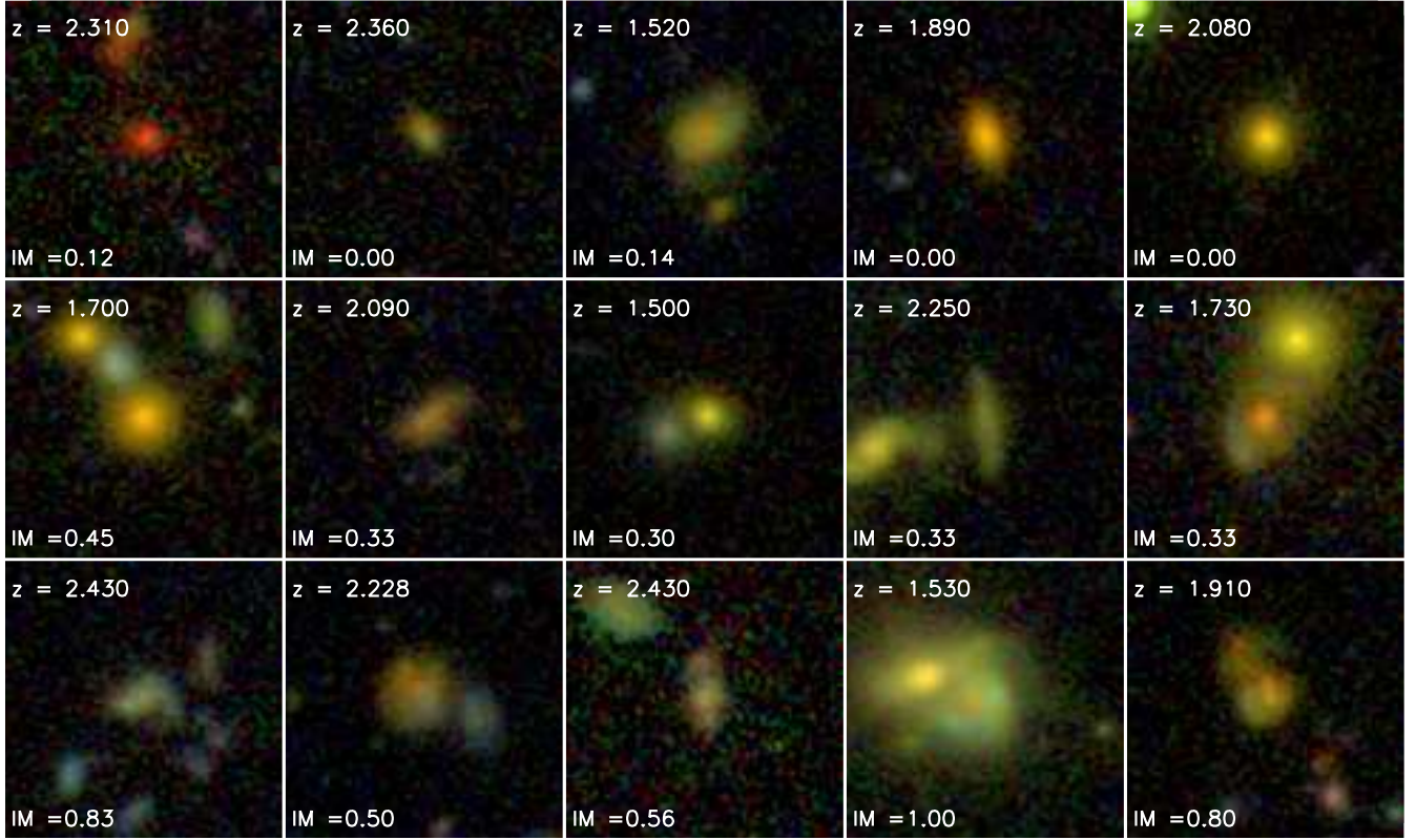
Fig. 2. A montage of randomly chosen inactive galaxies at 1.5 < z < 2.5 arranged in the fiducial bins of the visual Interaction Metric ( IM ). Each row of five galaxies are randomly selected from all objects in one of the three bins in IM (see Section 2.1.2). A redshift is written at the upper left of each panel and IM is written at the lower left. All three color (iJH) images are 6'' on a side and are identically scaled with a \sinh^{-1} stretch.
