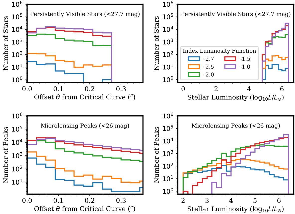
Extended Data Fig. 6: Offsets from critical curve and luminosities of lensed stars for different luminosity functions from 10^6 Monte Carlo simulations. We use the surface brightness ( F125W \approx 25 \text{ mag arcsec}^{-2} ) measured along the 0.2'' -wide arc to constrain the normalization of the stellar luminosity function, and then Poisson statistics to populate the source plane. The lower luminosity limit used for these simulations is 10 L_{\odot} . Upper panels show that stars with F125W \leq 27.7 \text{ mag} over a period lasting many years should only appear within \sim 0.15'' of the critical curve, and have luminosities of \gtrsim 10^{5.4} L_{\odot} . Lower panels show expected offset distribution of bright microlensing peaks ( F125W \leq 26 \text{ mag} ) to 0.4'' , and of the luminosities of lensed stars. A stellar luminosity function similar to that measured in nearby galaxies ( \alpha = -2.53 \pm 0.08 ) yields fewer events with less-luminous stars 20 . Left panels indicate the offset \theta in arcseconds of stars from the critical curve, while right panels show the intrinsic luminosity of the stars in units of the solar luminosity ( L_{\odot} ).
