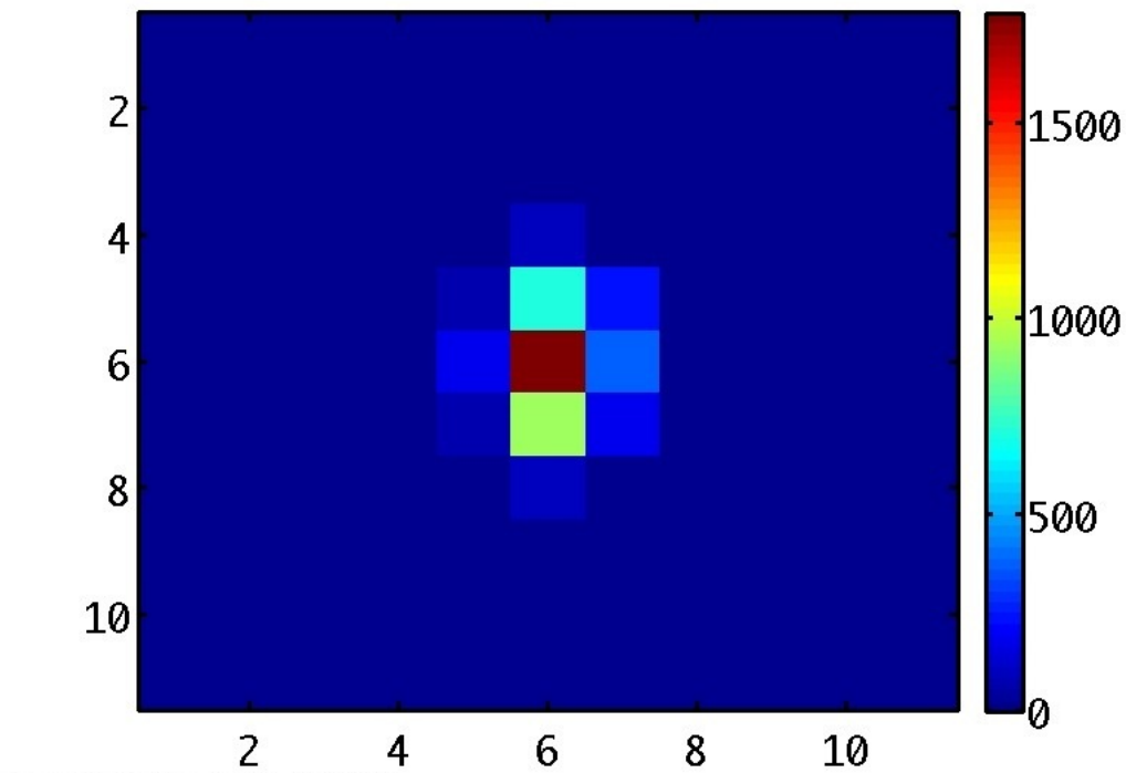
Figure 6: ALDEBARAH image in M band (Linear scale)
