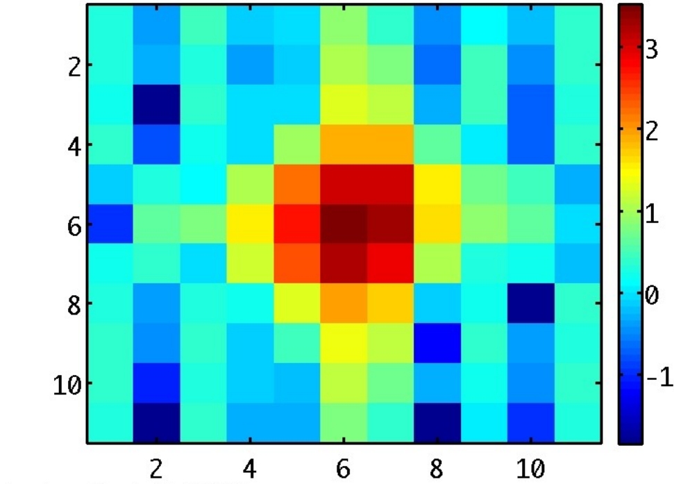
Figure 5:ALDEBARAH image in L band (Logarithmic scale)
