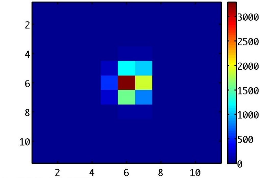
Figure 4: ALDEBARAH image in L band (linear scale)
