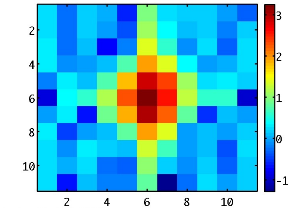
Figure 7: ALDEBARAH image in M band (Logarithmic scale)
