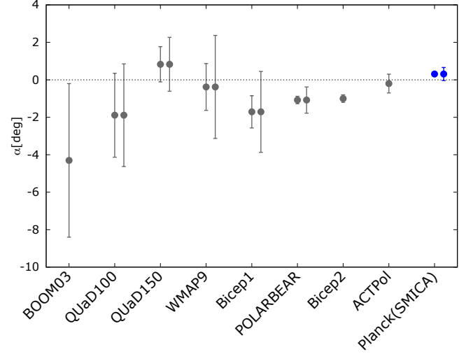
Fig. 8. Constraints on \alpha coming from published analyses of several sets of CMB experimental data sets (shown in grey) as reviewed in Kaufman et al. (2016) compared with what is found in the present paper (in blue). For each experiment the left error bars are for statistical uncertainties at 68% CL, while right error bars (when displayed) are obtained by summing linearly the statistical and systematic uncertainties. The error bar of BOOM03 already contains a contribution from systematic effects.
