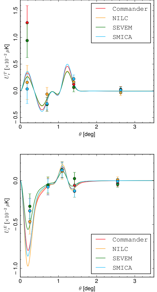
Fig. 3. Profiles of U_r from stacking on temperature (top) and E -mode (bottom) extrema for the four component-separation methods. The best-fit curves for each component-separation method are also shown, with \alpha values given in the fourth column of Table 1. Note that we have included both hot and cold spots in this figure, i.e., we have co-added the negative of the profile from cold spots to the profile of the hot spots. Error bars correspond to 68% confidence regions.
