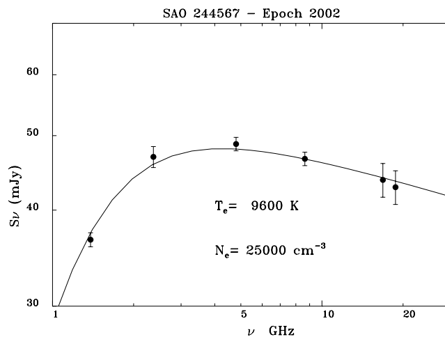
Figure 4. The observed flux densities superimposed to the radio spectrum of SAO 244567 obtained assuming a shell, 0.75 arcsec thick, with decreasing density ( \propto r^{-2} ), with T = 9600 K and n = 2.5 \times 10^4 \text{ cm}^{-3} at the inner radius.
