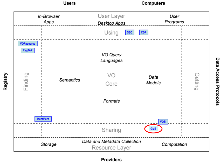
Figure 1: GMS in relation to the IVOA architecture
