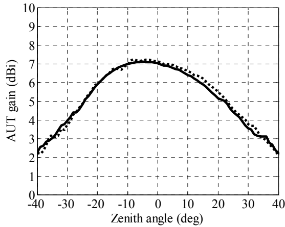
Figure 3: measured E-plane co-polar pattern at 350 MHz. Measurement with 0^\circ test-source orientation (dotted), measurement with 180^\circ test-source orientation (solid).
