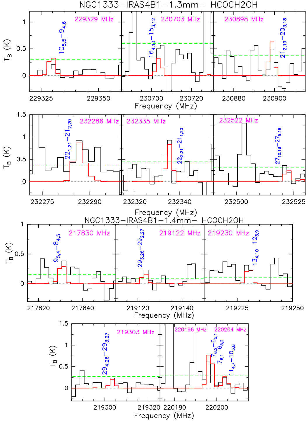
Fig. A.5. Glycolaldehyde emission lines (in T_B scale) detected in the 1.3mm and 1.4mm spectral windows towards NGC1333-IRAS4B1 and used to perform the LTE analysis. The horizontal green dotted lines show the 3\sigma level. In blue we mark the glycolaldehyde lines extracted from Table A.3. The red line shows the synthetic spectrum obtained with the GILDAS-Weeds package (Maret et al. 2011) and assuming the rotation diagram solutions (see Fig. 3).
