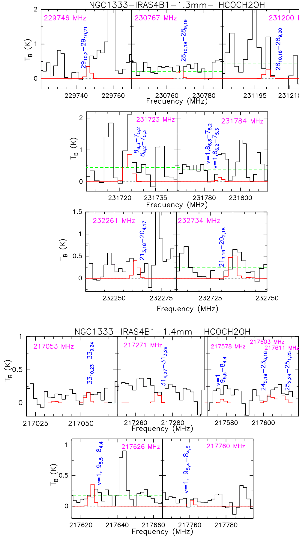
Fig. A.6. Glycolaldehyde emission lines (in T_B scale) observed in the 1.3mm and 1.4mm spectral windows towards NGC1333-IRAS4B1 and excluded from the LTE analysis because of severe blending with other emission lines. The horizontal green dotted lines show the 3\sigma level. In blue we mark the glycolaldehyde transitions. The red line shows the synthetic spectrum obtained with the GILDAS–Weeds package (Maret et al. 2011) and assuming the rotation diagram solutions (see Fig. 3).
