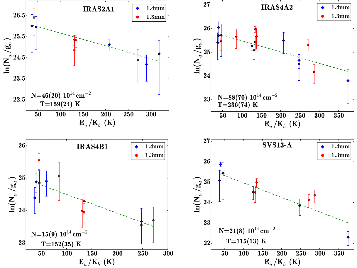
Fig. 3. Rotation diagram for the glycolaldehyde transitions reported in Table 2 for NGC1333-IRAS2A ( Upper-left panel ), NGC1333-IRAS4A2 ( Upper-right panel ), NGC1333-IRAS4B1 ( Lower-left panel ), and NGC133-SVS13A ( Lower-right panel ). The line intensities have been corrected for beam dilution using the sizes derived in Sect. 4.1. The parameters N_{\text{up}} , g_{\text{up}} , and E_{\text{up}} are respectively the column density, the degeneracy, and the energy of the upper level. The error bars on \ln(N_{\text{up}}/g_{\text{up}}) are given by the vertical bar of the symbols. Red and blue points refer to the lines detected in the 1.3 mm and 1.4 mm spectral bands, respectively. The dashed lines represent the best fits.
