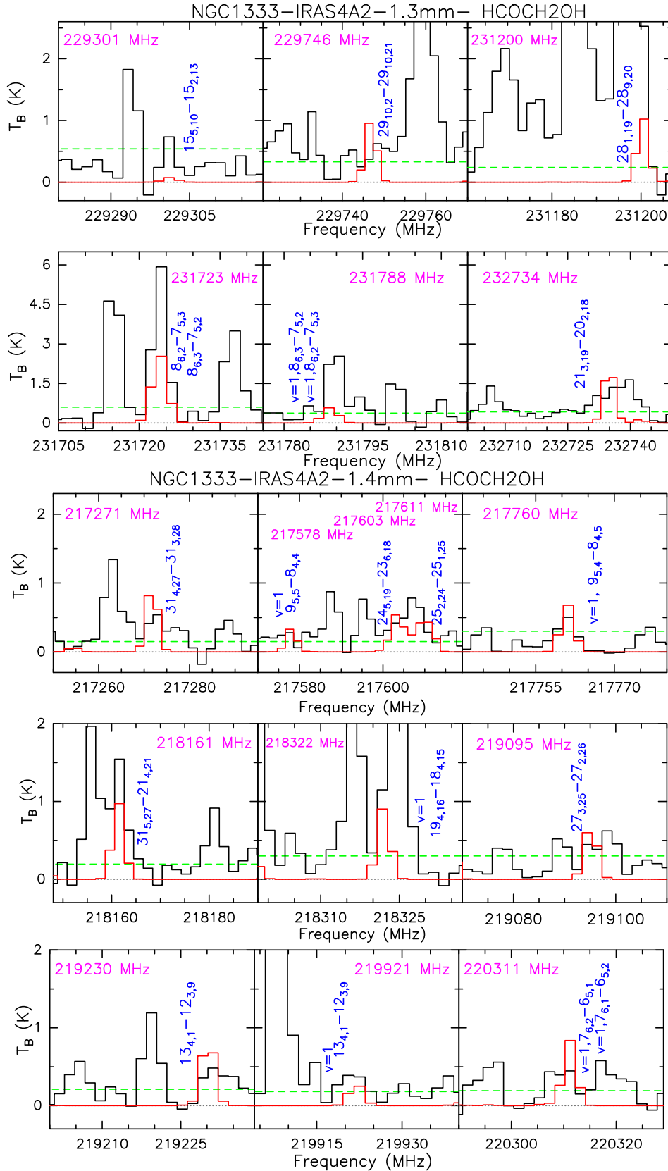
Fig. A.4. Glycolaldehyde emission lines (in T_B scale) observed in the 1.3mm and 1.4mm spectral windows towards NGC1333-IRAS4A2 and excluded from the LTE analysis because of severe blending with other emission lines. The horizontal green dotted lines show the 3\sigma level. In blue we mark the glycolaldehyde transitions. The red line shows the synthetic spectrum obtained with the GILDAS–Weeds package (Maret et al. 2011) and assuming the rotation diagram solutions (see Fig. 3).
