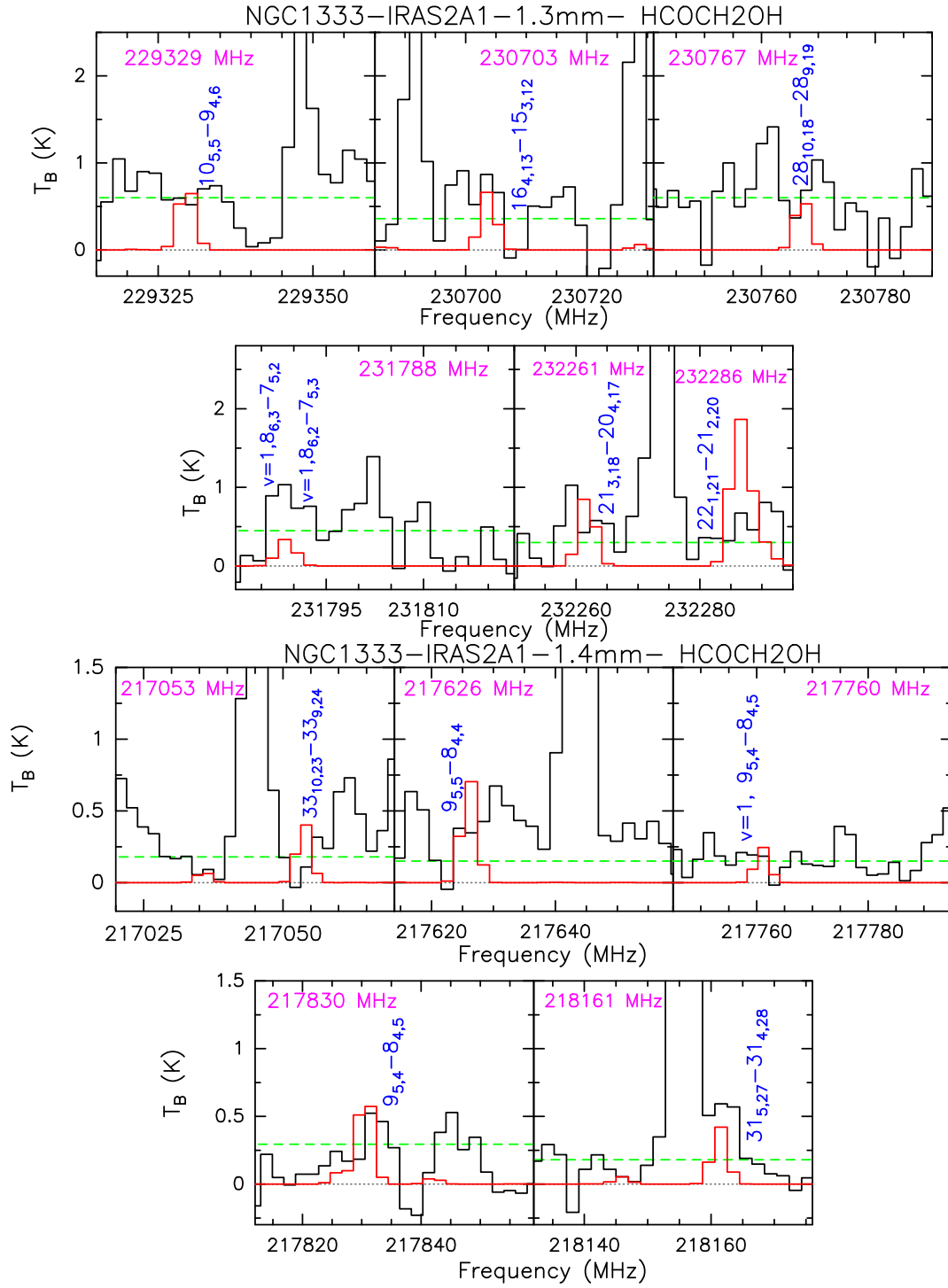
Fig. A.2. Glycolaldehyde emission lines (in T_B scale) observed in the 1.3mm and 1.4mm spectral windows towards NGC1333-IRAS2A1 and excluded from the LTE analysis because of severe blending with other emission lines. The horizontal green dotted lines show the 3\sigma level. In blue we mark the glycolaldehyde transitions. The red line shows the synthetic spectrum obtained with the GILDAS-Weeds package (Maret et al. 2011) and assuming the rotation diagram solutions (see Fig. 3).
