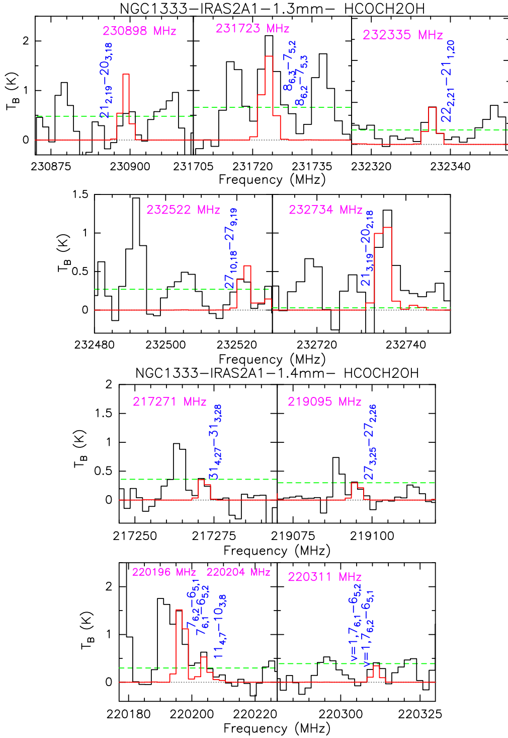
Fig. A.1. Glycolaldehyde emission lines (in T_B scale) detected in the 1.3mm and 1.4mm spectral windows towards NGC1333-IRAS2A1 and used to perform the LTE analysis. The horizontal green dotted lines show the 3\sigma level. In blue we mark the glycolaldehyde lines extracted from Table A.1. The red line shows the synthetic spectrum obtained with the GILDAS–Weeds package (Maret et al. 2011) and assuming the rotation diagram solutions (see Fig. 3).
