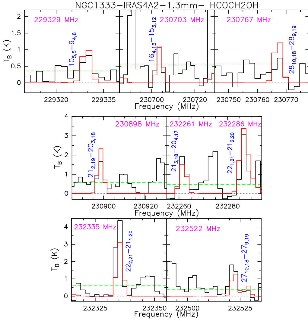
Fig. A.3. Glycolaldehyde emission lines (in T_B scale) detected in the 1.3mm and 1.4mm spectral windows towards NGC1333-IRAS4A2 and used to perform the LTE analysis. The horizontal green dotted lines show the 3\sigma level. In blue we mark the glycolaldehyde lines extracted from Table A.2. The red line shows the synthetic spectrum obtained with the GILDAS-Weeds package (Maret et al. 2011) and assuming the rotation diagram solutions (see Fig. 3).
