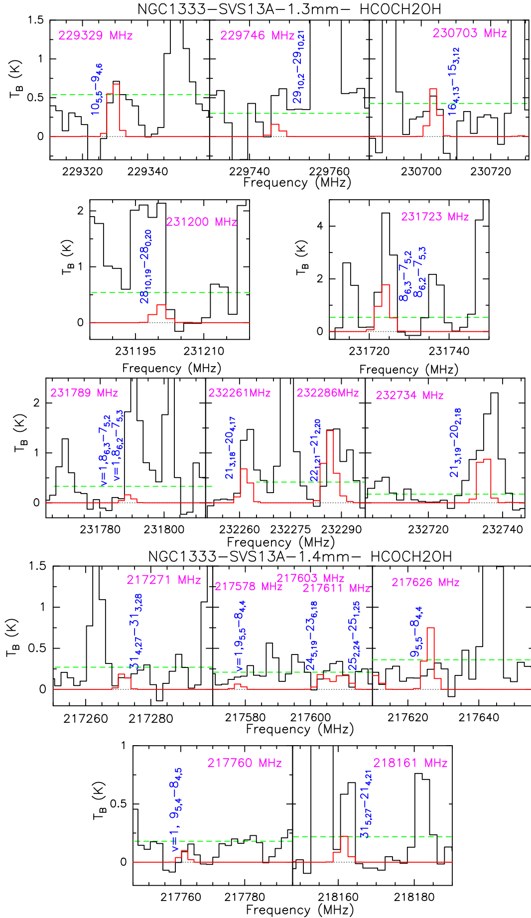
Fig. A.8. Glycolaldehyde emission lines (in T_B scale) observed in the 1.3mm and 1.4mm spectral windows towards NGC1333-SVS13A and excluded from the LTE analysis because of severe blending with other emission lines. The horizontal green dotted lines show the 3\sigma level. In blue we mark the glycolaldehyde transitions. The red line shows the synthetic spectrum obtained with the GILDAS–Weedle package (Marrone et al. 2012) and assuming the rotation diagram solutions (see Fig. 3).
