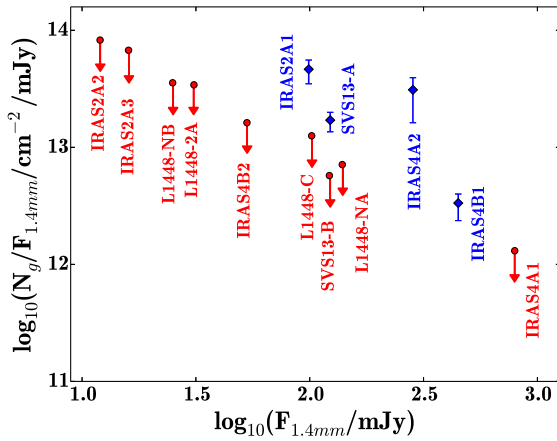
Fig. 5. Ratio between the glycolaldehyde column density ( N_{\text{tot}} ) and the peak flux of the 1.4mm continuum emission ( F_{1.4\text{mm}} ; Maury et al., in preparation) versus the 1.4mm peak flux. Red arrows are for sources where glycolaldehyde has not been detected.
