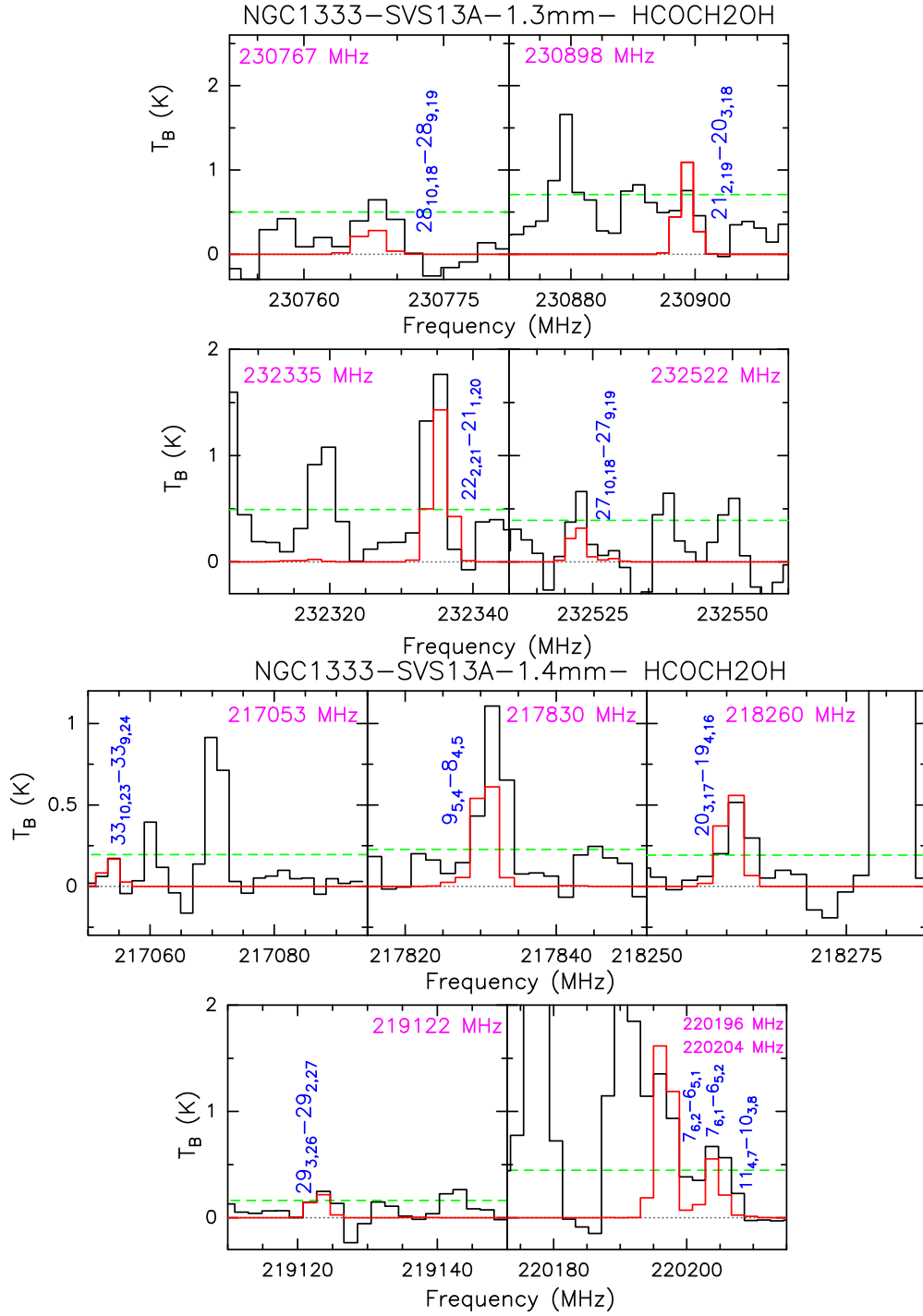
Fig. A.7. Glycolaldehyde emission lines (in T_B scale) detected in the 1.3mm and 1.4mm spectral windows towards NGC1333-SVS13A and used to perform the LTE analysis. The horizontal green dotted lines show the 3\sigma level. In blue we mark the glycolaldehyde lines extracted from Table A.4. The red line shows the synthetic spectrum obtained with the GILDAS-Weeds package (Maret et al. 2011) and assuming the rotation diagram solutions (see Fig. 3).
