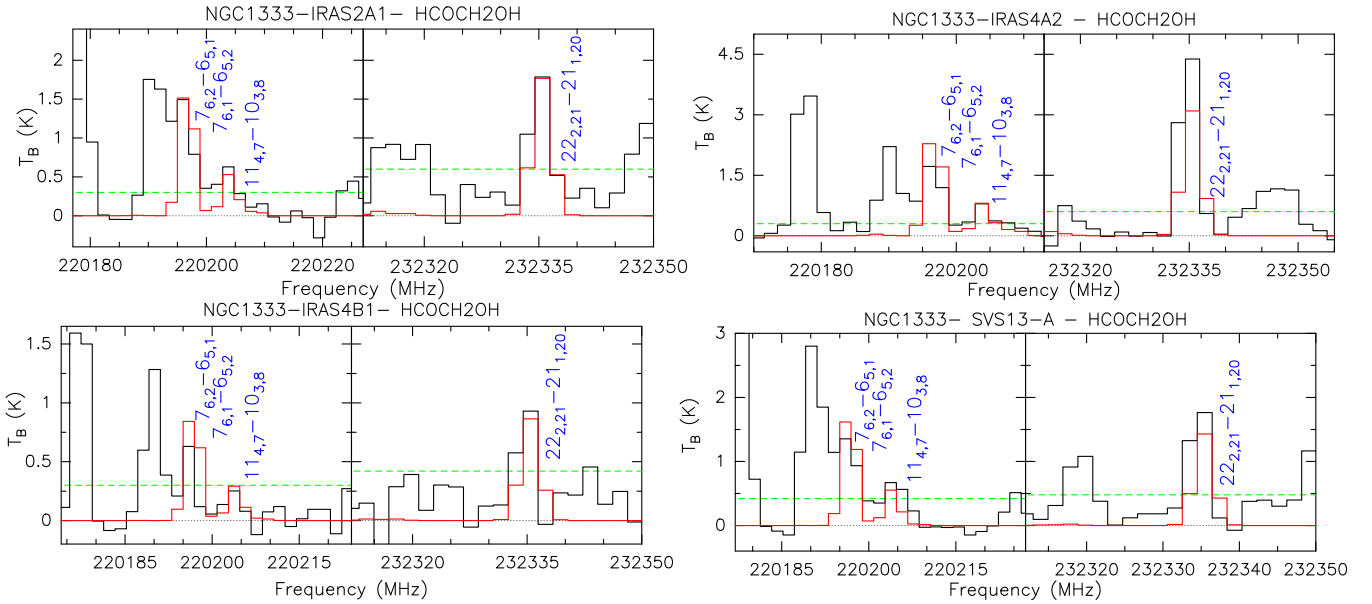
Fig. 1. Examples of glycolaldehyde emission lines (in T_B scale) observed in the 1.3mm and 1.4mm spectral windows (and at different upper-level energy, E_u from 37 K to 135 K) towards NGC1333-IRAS2A1 (Upper-left panel), NGC1333-IRAS4A2 (Upper-right panel), NGC1333-IRAS4B1 (Lower-left panel), and NGC1333-SVS13A (Lower-right panel). The horizontal green dotted lines show the 3\sigma level. In blue we mark the glycolaldehyde lines extracted from Tables A1-A4. The bright line at \sim 220190 MHz is due to \text{CH}_3\text{OCHO}(17_{4,13}-16_{4,12})\text{A} (Maury et al. 2014; Belloche et al. in preparation). The red line shows the synthetic spectrum obtained with the GILDAS-Weeds package (Maret et al. 2011) and assuming the rotation diagram solutions (see Fig. 3).
