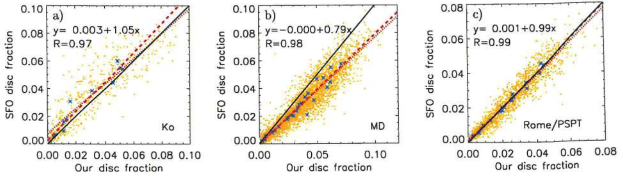
Fig. 13. Same as Fig. 12, but now comparing the plaque areas derived by SFO ( y -axis) and those obtained here ( x -axis): (a): Ko data; (b): MD data; (c): Rome/PSPT data.
