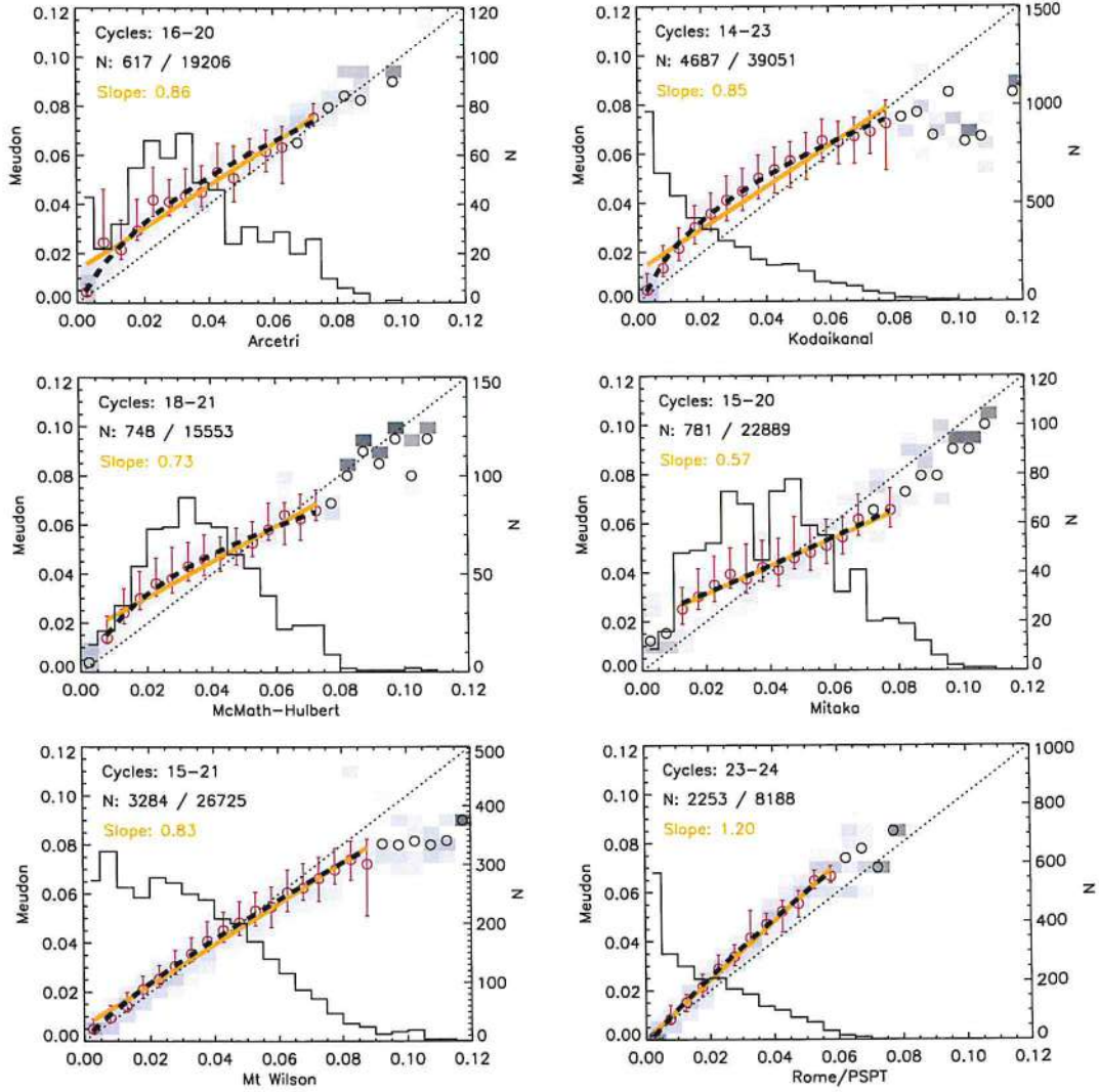
Fig. 10. Same as Fig. 7, but with MD plate area series as reference and Ar, Ko, MM, Mi, MW, and Rome/PSPT series as the secondary, by considering the whole period of observations over which the respective datasets overlap (see Table 2).
