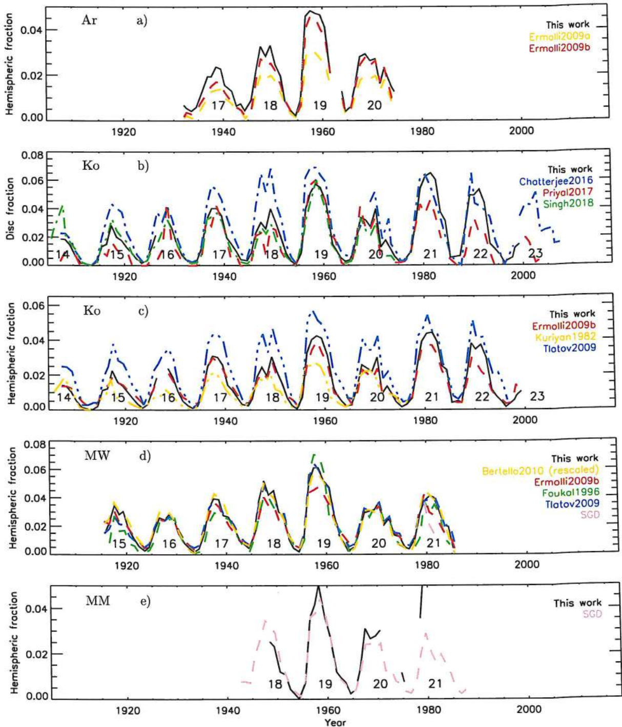
Fig. 11. Comparison of the plage areas derived here (black) to other published series based on the same datasets. (a): Ermolli et al. (2009a, yellow) and Ermolli et al. (2009b, red) for Ar data; (b): Chatterjee et al. (2016, blue), Priyal et al. (2017, red), and Singh et al. (2018, green) for Ko areas in disc fractions; (c): Ermolli et al. (2009b, red), Kuriyan et al. (1982, yellow), and Tlatov et al. (2009, blue) for Ko areas in fractions of a hemisphere; (d): Bertello et al. (2010, yellow), Ermolli et al. (2009b, red), Foukal (1996, green), Tlatov et al. (2009, blue), and SGD (pink) for MW data; (e): SGD (pink) for MM data. The curves are annual median values. All panels except (b) are in fractions of hemisphere corrected for projection effects. The numbers under the curves denote the conventional SC numbering.
