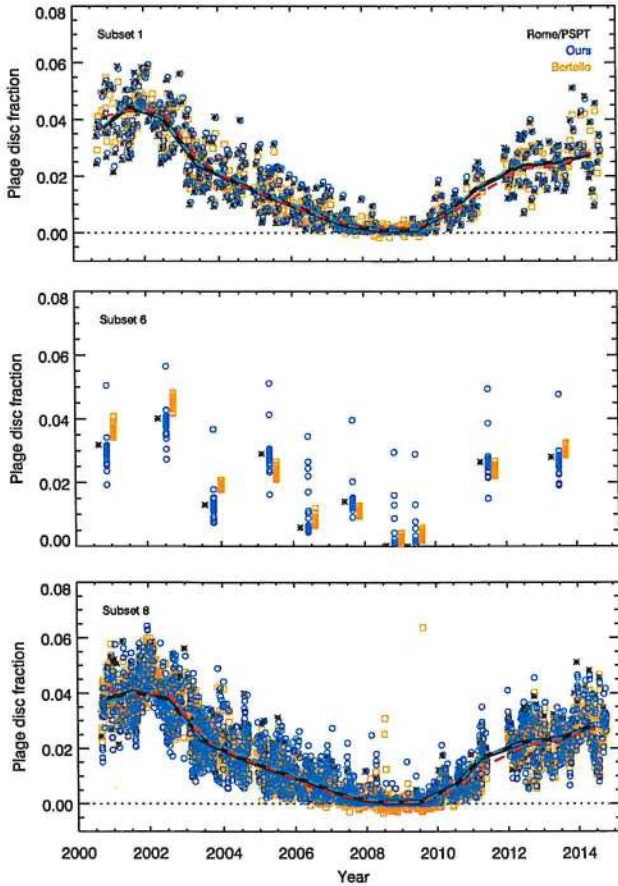
Fig. 15. Comparison between plate area disc fractions derived with our method (blue circles) and that by Bertello et al. (2010, orange squares) for subset 1 (top), subset 6 (middle), and subset 8 (bottom). The disc fraction from the original Rome/PSPT data used to create the synthetic images are shown as black asterisks. The blue circles lie almost perfectly over the black asterisks for subset 1. To improve the visibility of the results for subset 6, the plate areas derived with our method and those by Bertello et al. (2010) have been shifted in the x-axis by 0.2 yr and 0.4 yr, respectively. Annual median values are shown for the original Rome/PSPT data (solid black line) and for the synthetic data processed with our method (dashed light blue line) and Bertello et al. (2010, dashed red line). The dotted black horizontal line is for plate area disc fraction of 0. Subset 6 is only available for 10 days during the considered period. The negative values of plate areas obtained with the method by Bertello et al. (2010) are due to the linear scaling applied to match the results to the original Rome/PSPT plate areas, see Sect. 5.2 for more information.
