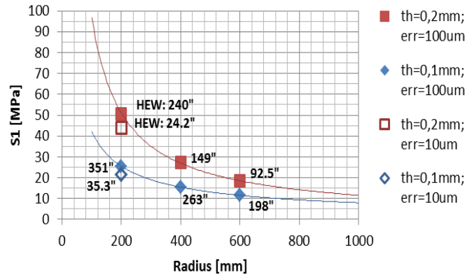
Figure 3: Maximum stress in a flat glass integrated with cold slumping approach after the vacuum release, and expected HEW of the integrated samples
