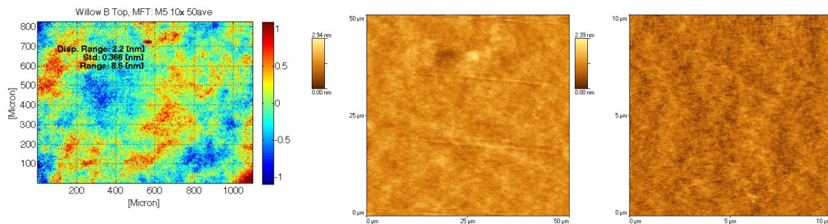
Figure 6: (A) An example of the images (color scale in nm) acquired on the Willow surface with the MFT (10x objective). The surface is 0.366 nm rms on the mm scale. (B) and (C): the surface as observed with the AFM on 50microns and 10microns scale, with rms(50 \mu m)=0.23 nm, rms(10 \mu m)=0.24 nm. The color scale is always in nm.
