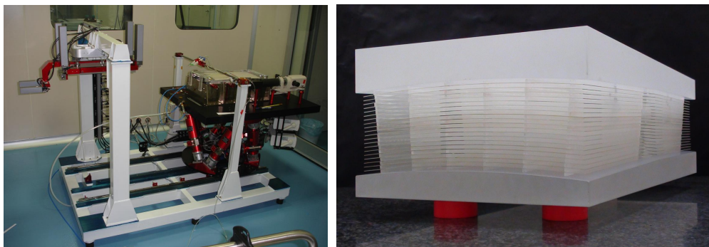
Figure 1: The Integration Machine (IMA) in INAF/OAB laboratories and the X-ray Optical Unit Breadboard (XOU_BB) [11]
