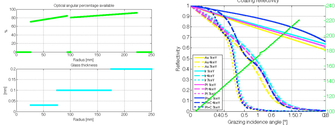
Figure 7: Left, Optical free angular percentage and glass thickness. The thickness is 30 microns, 100 microns and 200microns depending on the radius of curvature. Right, Coating Reflectivity versus incidence angle.
