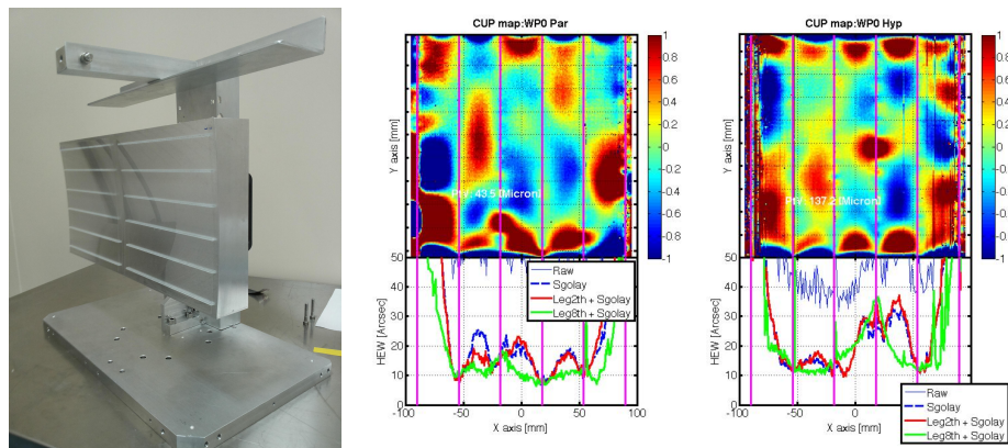
Figure 10: First integrated prototype based on thin glass cold slumping technology.
