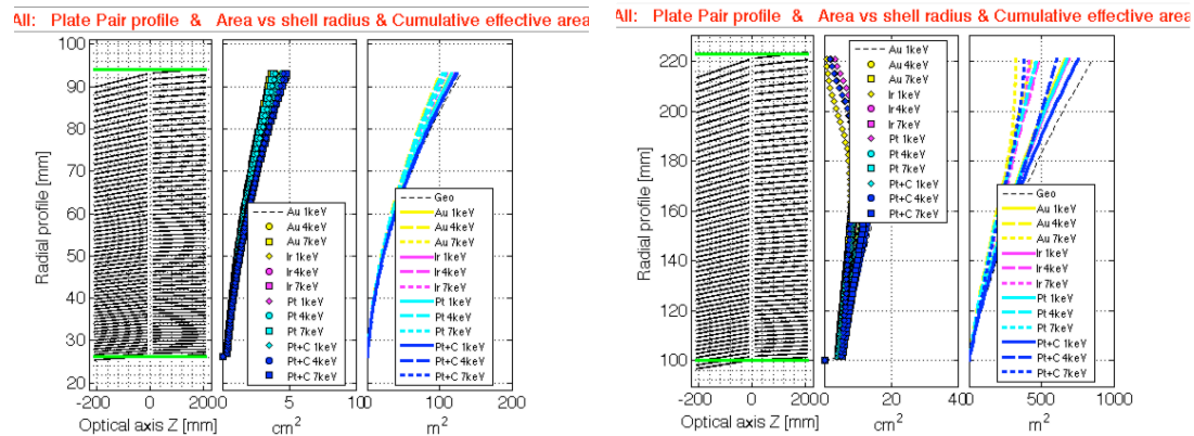
Figure 8: Mirror profiles, effective area per shell and cumulative area for inner and outer parts.
