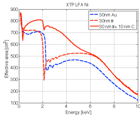
Figure 9: Effective area for a LFA module based electroformed nickel technology.
