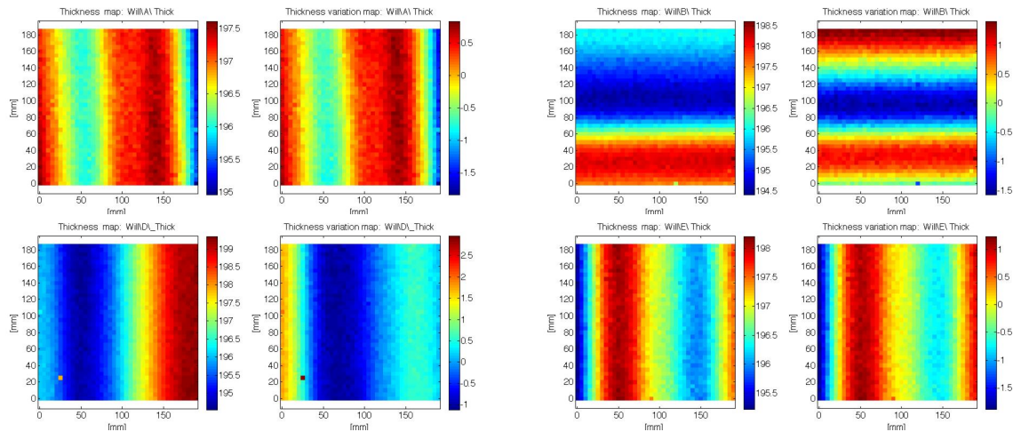
Figure 5: The thickness and the thickness variation as measured by the CUP on the four Willow samples. The color scale in the images is in microns.
