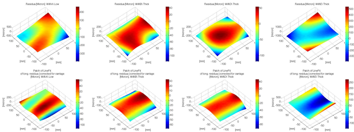
Figure 4: The residua with respect to a plane and along the vertical direction as measured on the four samples considered.
