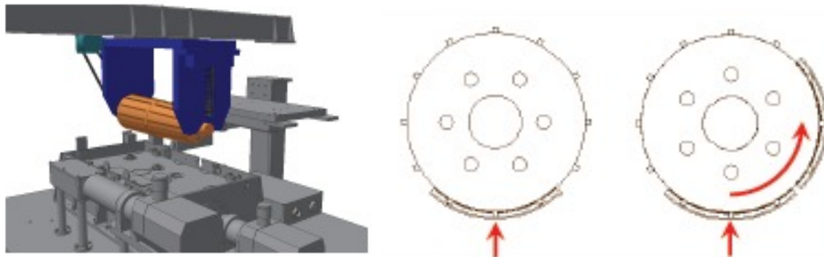
Figure 2: The changes in the IMA set-up to assemble mirror module with small radius of curvature: a rotary movement is introduced allowing the glass stacking around the central mandrel.
