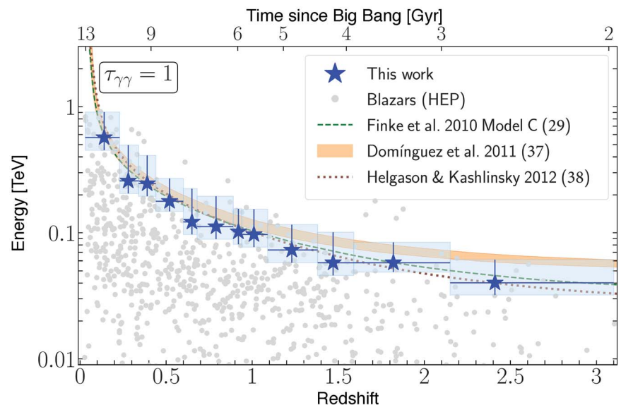
Fig. 1. The cosmic \gamma -ray horizon. Measurement of the cosmic \gamma -ray horizon ( \tau_{\gamma} = 1 , i.e., the point after which the Universe becomes opaque to \gamma rays) as a function of redshift (blue stars). Horizontal and vertical blue lines represent the redshift bin size and the uncertainty on the energy, respectively. Also shown are predictions from three different EBL models (29, 37, 38) for comparison. The gray points show the highest-energy photon (HEP) detected from each blazar considered in this work. Gyr, billions of years.
